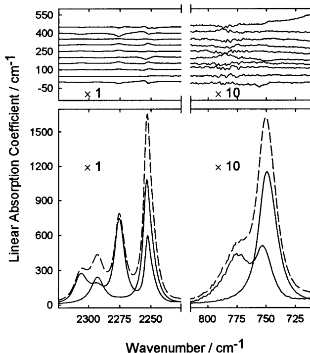
Figure 9. Multiple-dimensional curve fit of the ACN \nu_2 and 2\nu_8 spectral regions of \text{LiClO}_4 -ACN solutions based the model encompassed by eqs 1 and 2 in the text and using a value of the total number of solvent molecules influence by both \text{ClO}_4^- and the \text{Li}^+ cation of 8. (top) Residuals (offset for clarity) are shown for the curve fits of the spectra shown in Figure 1. The bottom-most residual is from the curve fit of the pure ACN spectrum, and each successive residual is from the curve fit of the spectrum of greater \text{LiClO}_4 concentration (concentrations given in Figure 1). (bottom) The curve fit of the 0.887 M \text{LiClO}_4 -ACN solution spectrum. The measured spectrum is indicated with a dashed line.
