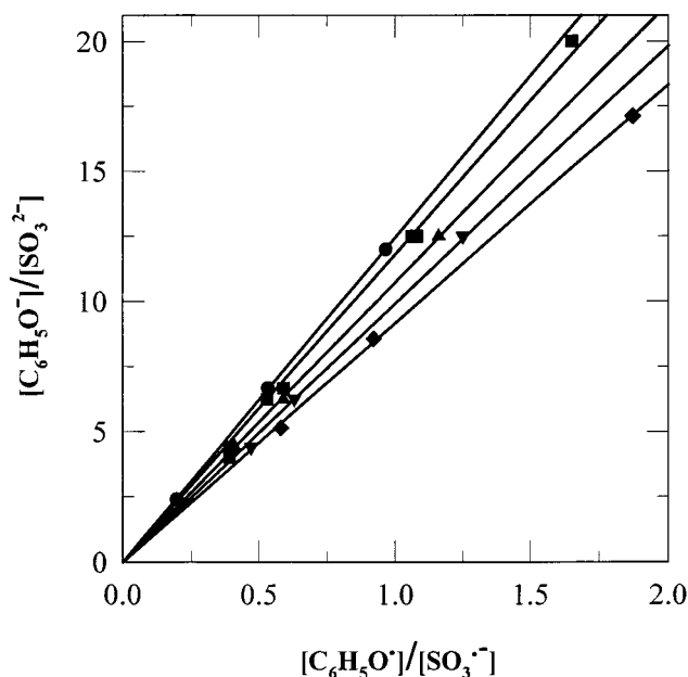
Figure 3. Variation of K for the equilibrium between \text{C}_6\text{H}_5\text{O}^-/\text{C}_6\text{H}_5\text{O}^{\bullet-} and \text{SO}_3^{\bullet-}/\text{SO}_3^{2-} in \text{N}_2\text{O} -saturated solutions at different I values, absorbed dose \sim 5 Gy. The solution compositions for ( \bullet ) I = 67 mmol \text{L}^{-1} , ( \blacksquare ) I = 92 mmol \text{L}^{-1} , ( \blacktriangle ) I = 192 mmol \text{L}^{-1} , ( \blacktriangledown ) I = 342 mmol \text{L}^{-1} , and ( \blacklozenge ) I = 855 mmol \text{L}^{-1} are listed in Table 2.
