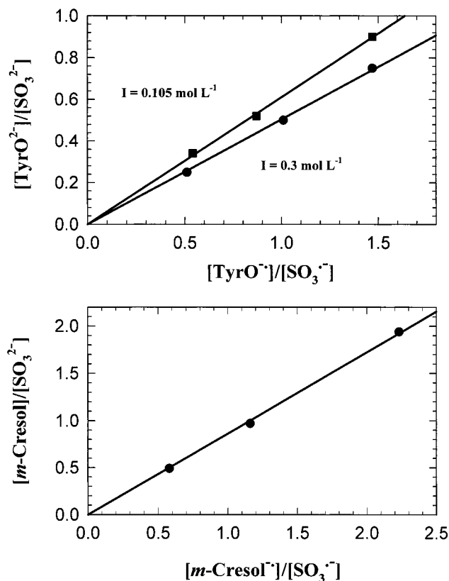
Figure 2. Measurement of the equilibrium constants for the reactions \text{TyrO}^- + \text{SO}_3^{2-} \rightleftharpoons \text{TyrO}^{\bullet-} + \text{SO}_3^{\bullet-} and \text{m-Cresol}^- + \text{SO}_3^{2-} \rightleftharpoons \text{m-Cresol}^{\bullet-} + \text{SO}_3^{\bullet-} .
