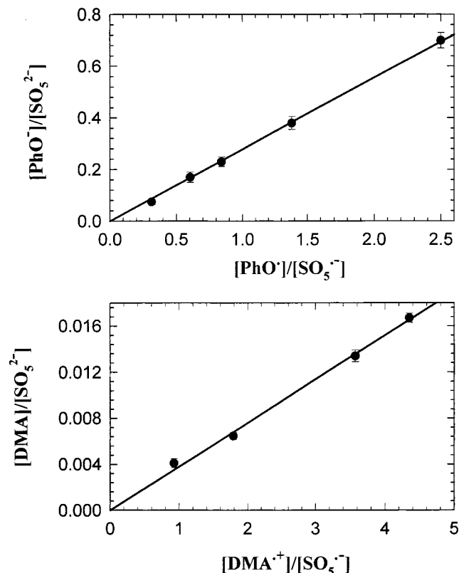
Figure 6. Measurement of the equilibrium constants for the reactions \text{PhO}^\bullet + \text{SO}_5^{2-} \rightleftharpoons \text{PhO}^- + \text{SO}_5^{\cdot-} and \text{DMA}^{\cdot+} + \text{SO}_5^{2-} \rightleftharpoons \text{DMA} + \text{SO}_5^{\cdot-} .
