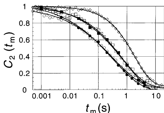
Figure 8. Semilog plot of the correlation function C_2(t_m) versus mixing time t_m for benzene/Ag–Y. Data acquired at 193 K (circles) and 183 K (squares) were obtained both from static 2D exchange ^{13}\text{C} NMR spectra (filled symbols) and ^{13}\text{C} stimulated echoes with t_e = 50 \mu\text{s} (open symbols), showing excellent agreement between the two methods. The shape of the decay of C_2(t_m) measured at 153 K using stimulated echoes (open diamonds) more closely resembles a single exponential than the higher-temperature data. This change in shape at low temperature is consistent with the onset of spin diffusion, indicating that at 183 and 193 K molecular reorientation is the dominant process contributing to ^{13}\text{C} NMR frequency changes.
