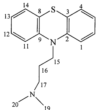
Figure 1. Diagram of the promazine molecule with the carbon and nitrogen atoms numbered 1–20.
