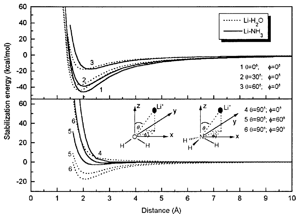
Figure 4. Comparison of the \text{Li}^+ - \text{H}_2\text{O} and \text{Li}^+ - \text{NH}_3 interaction energies for some values of \theta and \phi , obtained from the ab initio calculations with double- \zeta valence basis set.
