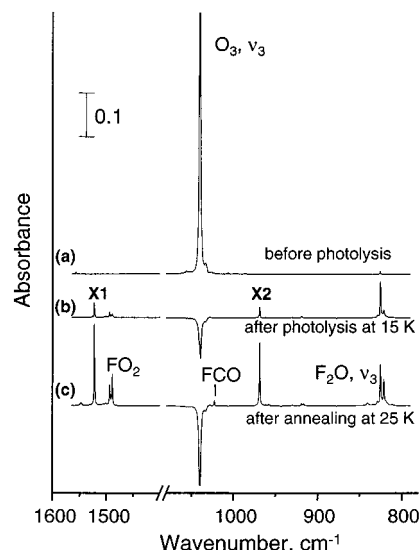
Figure 2. Infrared spectra of the sample Ar:F 2 :O 3 = 5000:3:1 at 15 K. Trace a shows the structure of the O 3 band prior to photolysis. Trace b is a difference spectrum showing changes in the bands following 355 nm photolysis at 15 K. Trace c is a difference spectrum showing the additional changes that occur during annealing of the sample at 25 K.
