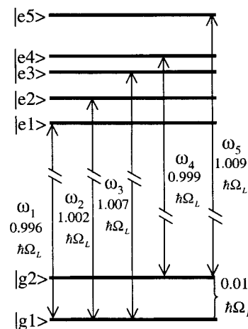
Figure 4. Energy level diagram of the seven level system used in this simulation in section 4.2.1. In equation 23 the corresponding Hamiltonian is given in the rotating picture with V = -1/2A\mu . A is the amplitude of the square laser pulse envelope and \mu is the effective transition dipole moments (set at 1 D in this simulation).
