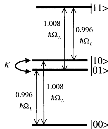
Figure 6. Energy level diagram for two chromophores coupled through interaction \kappa . The states are in the local excitation basis. The Hamiltonian describing the system is given in eq 24.
