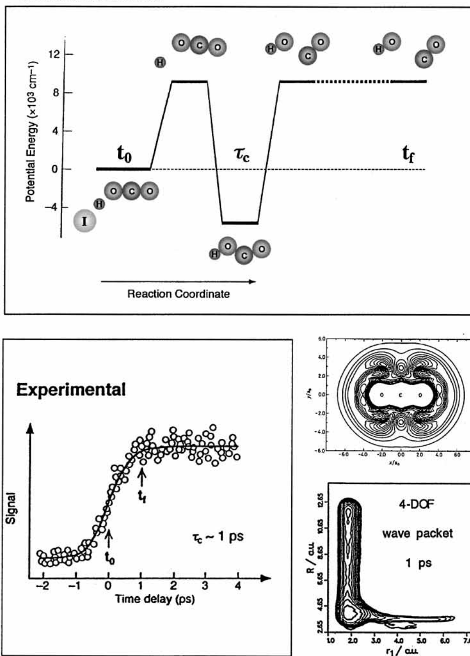
Figure 10. Femochemistry of the bimolecular \text{H} + \text{CO}_2 reaction. The precursor in this molecular beam experiment is \text{HI}/\text{CO}_2 in a van der Waals complex. The initial experiments utilized picosecond pulses, but later subpicosecond pulses were used (see text). Theoretical ab initio calculations of the PES and the dynamics (classical, semiclassical and quantum wave packet) have all been reported (see text). The transit species \text{HOCO}^+ lives for \sim 1 ps. Similar studies were made of reactive \text{Br} + \text{I}_2 , of the inelastic collision between \text{I} and \text{CH}_3\text{I} , and of other bimolecular reactions. Reference 45.
