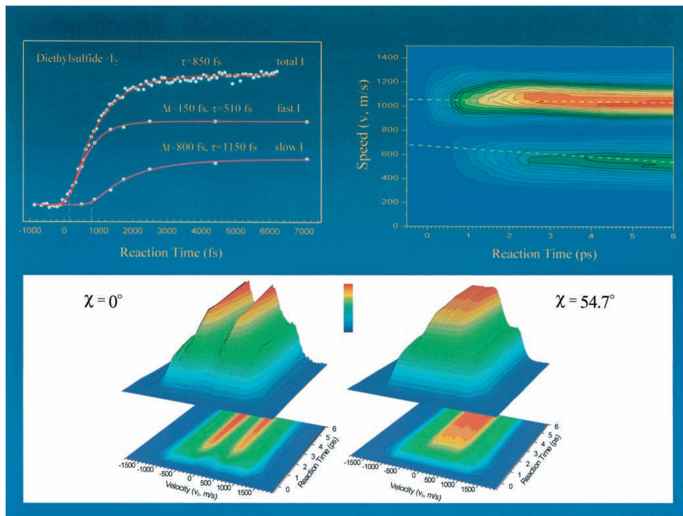
Figure 13. Femtochemistry of bimolecular electron-transfer reactions, the classic case of donors (e.g., benzene or diethyl sulfide) and acceptors (e.g., iodine or iodomonochloride). The experimental results clearly show the distinct velocity and time correlations, and thus the two-speed distributions and time scales of the reaction on the global PES. Reference 47.
