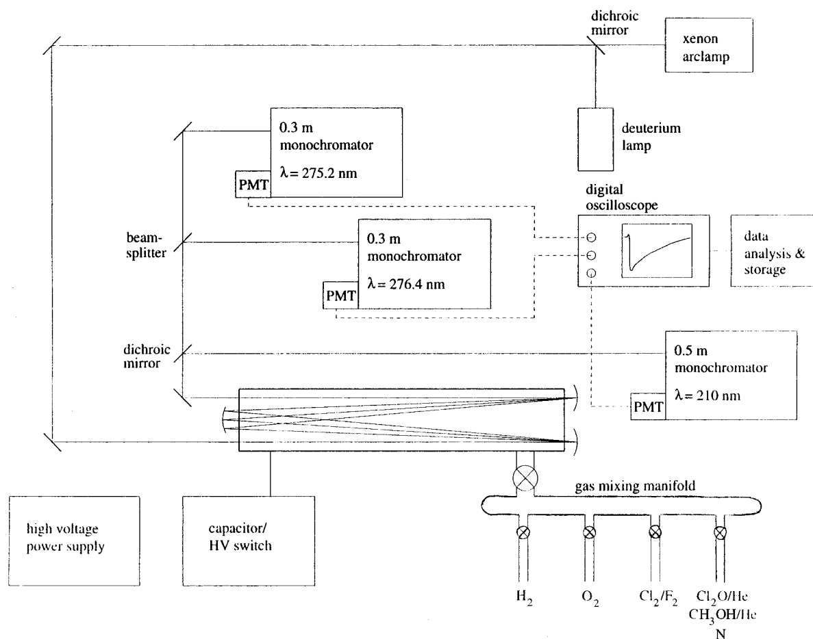
Figure 1. Schematic diagram of flash photolysis/ultraviolet absorption apparatus. The CW probe consists of a 150 W deuterium lamp and a 300 W xenon arc lamp combined with a dichroic beam splitter. Both probes traced the same 720 cm optical path within the flash photolysis cell. A second dichroic beam splitter at the exit separated the probes into a long-wavelength component for ClO detection and a short-wavelength component for HO 2 detection.
