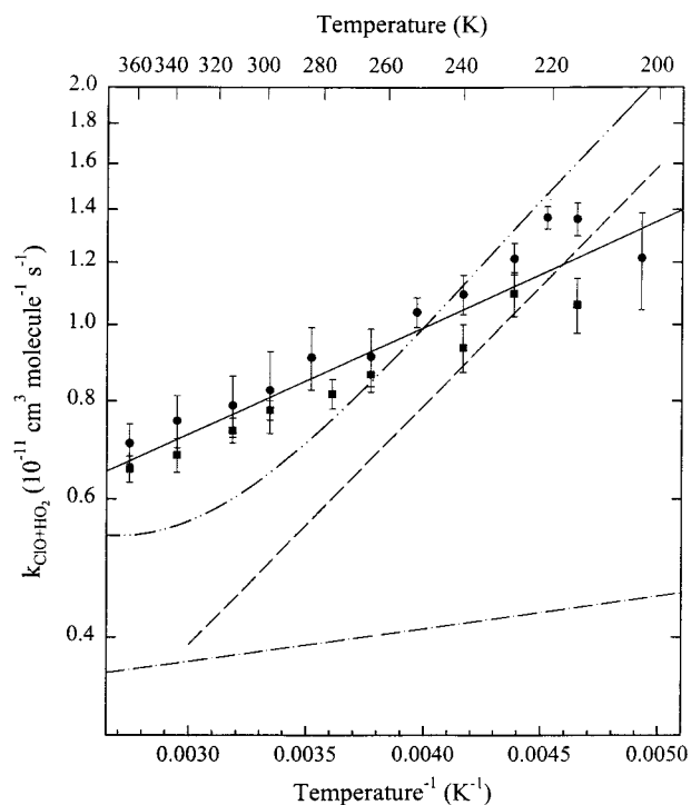
Figure 4. Arrhenius plot of temperature dependence data for the ClO + HO 2 reaction: (●) this work, data obtained using the F 2 –H 2 –O 2 –Cl 2 O system; (■) this work, data obtained using Cl 2 –CH 3 OH–O 2 –Cl 2 O system; (—) fit to the combined data from both chemical systems; (– · – ·) fit to the data of Stimpfle et al.; 7 (– – –) recommendation from JPL 97–4 Data Evaluation; 17 (○ – ○) data obtained using the discharge flow/mass spectrometry technique at 1 Torr from this laboratory. 34
