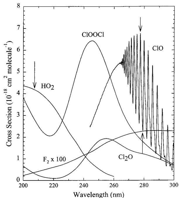
Figure 2. Absorption spectra of species involved in the HO 2 + ClO kinetics studies. Arrows denote the wavelengths used for the detection of HO 2 at 210 nm and ClO by differential absorption at 275 nm.
