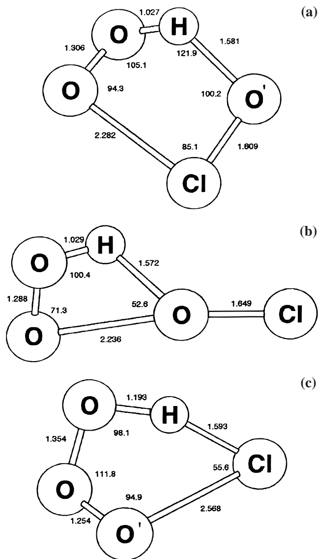
Figure 5. Transition state structures for reaction pathways on the singlet surface of the HO 2 + ClO reaction. Structures are calculated at the B3LYP/6-311++(3df,3pd) level of theory: (a) transition state for the pathway HOOCiO → HOCl + O 2 ( 1 Δ); (b) transition state for the pathway HOOCiCl → HOCl + O 2 ( 1 Δ); (c) transition state for the pathway HOOCiCl → HCl + O 3 .
