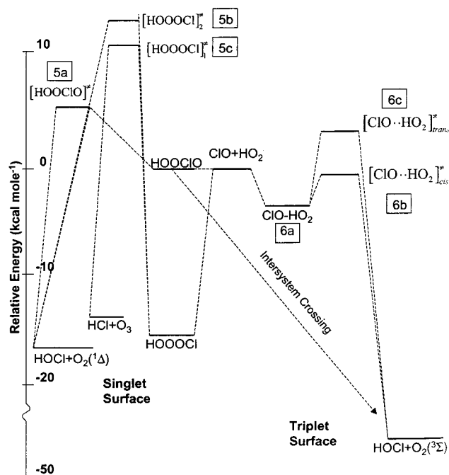
Figure 7. Schematic diagram showing energy levels and reaction pathways for the HO 2 + ClO reaction along the singlet and triplet pathways. Numbers next to chemical symbols refer to the figures showing the corresponding structures.
