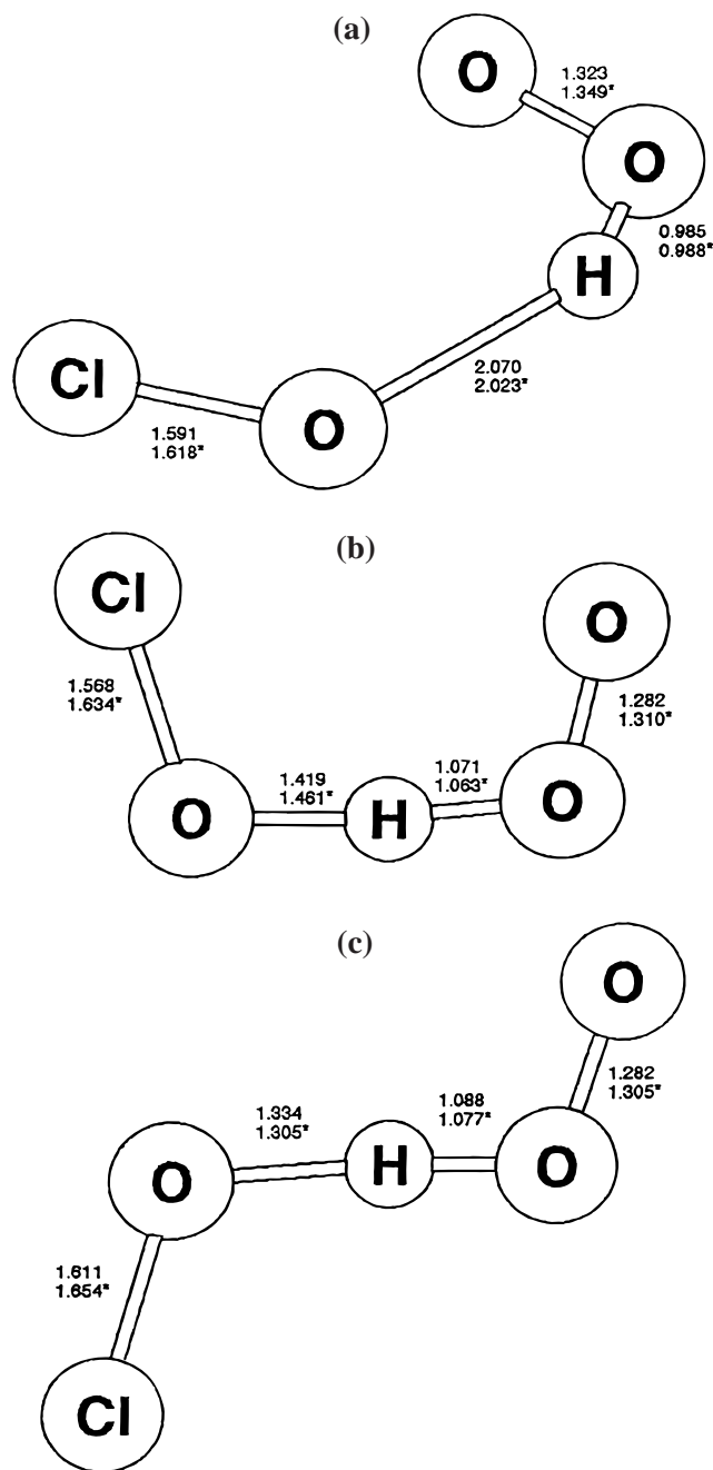
Figure 6. Transition state structures for reaction pathways on the triplet surface of the HO 2 + ClO reaction. Two values are given for each bond length. The upper value is the result obtained at the UMP2/6-31G(d) level of theory, while the lower value is obtained using the CCSD(T)/6-31G(d) level of theory: (a) triplet state complex; (b) cis transition state; (c) trans transition state.
