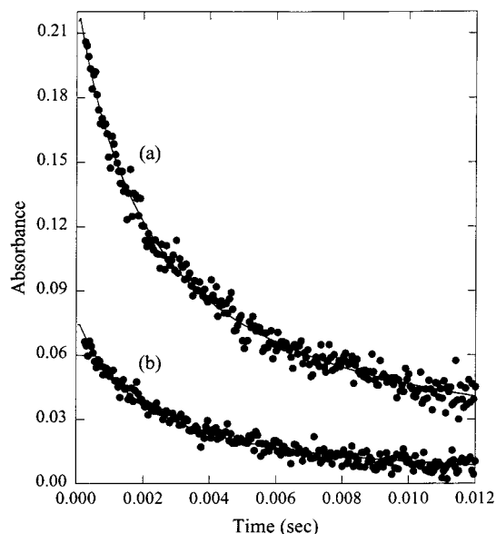
Figure 3. Example of time-resolved absorption signals for the F 2 -H 2 -O 2 -Cl 2 O system: (a) 210 nm absorption channel (HO 2 ); (b) differential absorption signal from 275.2 and 276.4 nm channels (ClO). The solid lines are fits obtained using FACSIMILE as discussed in the text.
