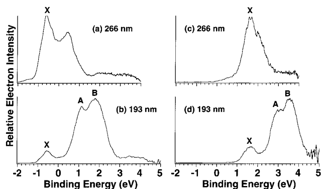
Figure 12. Photodetachment spectra of [\text{CuPc}(\text{SO}_3)_4]^{4-} and [\text{CuPc}(\text{SO}_3)_4\text{H}]^{3-} at 266 and 193 nm: (a, b) [\text{CuPc}(\text{SO}_3)_4]^{4-} ; (c, d) [\text{CuPc}(\text{SO}_3)_4\text{H}]^{3-} . Note the negative electron binding energy feature (X) of the tetraanion and the rigid shift to higher binding energies of the trianion spectra. From ref 18.
