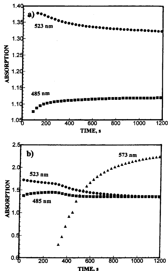
Figure 2. Kinetics of the absorption in water solutions of PIC at 2 \times 10^{-4} mol/L (a) and 3 \times 10^{-4} mol/L (b).
