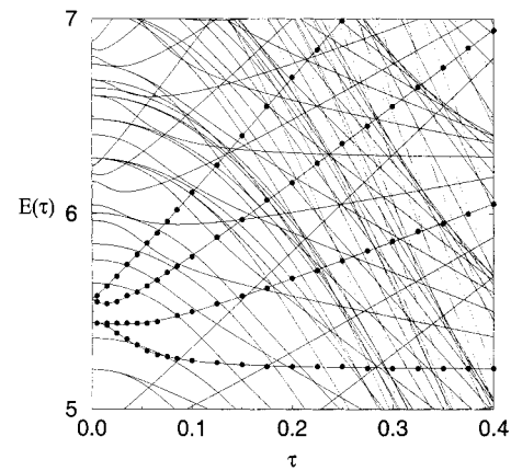
Figure 2. Level dynamics for the integrable 1:1 case. The fan formed by the states belonging to the polyad P = 6 is shown. The solid points correspond to resonant states as identified in the (I_1, I_2) space.
