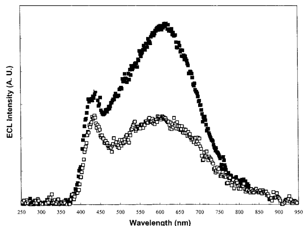
Figure 3. Electrogenerated chemiluminescence emission spectra of 3.3 \times 10^{-5} M (open squares) and 6 \times 10^{-5} M (filled squares) PDOF solutions in benzene:acetonitrile 9:1 containing 0.1 M TBAPF 6 as an electrolyte. All spectra were obtained with an integration time of 10 min.
