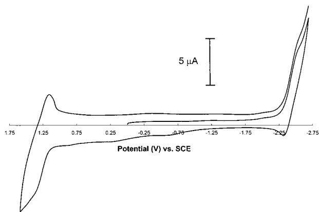
Figure 2. Cyclic voltammogram of 6 \times 10^{-5} M polyfluorene in 9:1 benzene:CH 3 CN 9:1 containing 0.1 M TBAPF 6 as an electrolyte with a scan rate of 0.5 V/s.
