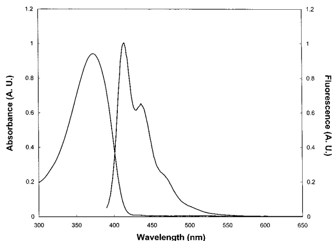
Figure 1. Absorption and fluorescence spectra of 3.3 \times 10^{-5} M PDOF solution in benzene:MeCN 9:1 taken with a 1 mm cuvette under atmospheric conditions. \lambda_{exc} = 380 nm.
