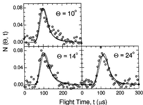
Figure 5. TOF spectra of the ND product from the N(^2D) + D_2 reaction at E_c = 5.1 \text{ kcal mol}^{-1} . Solid and dashed lines as defined in Figure 2.
