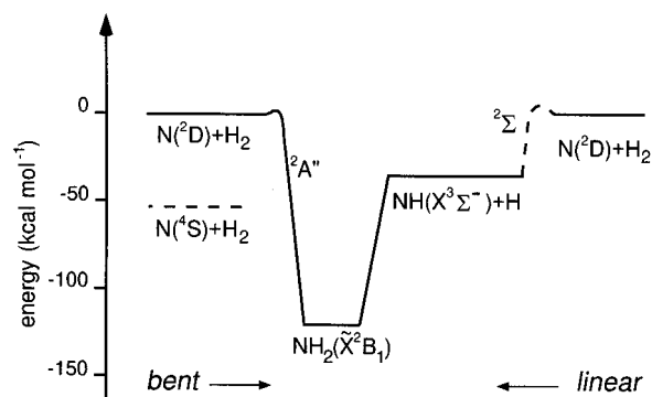
Figure 1. Schematic energy level and correlation diagram for the reaction N(^2D) + H_2 based on ab initio electronic structure calculations of the ground PES. Both bent and linear geometries are shown.
