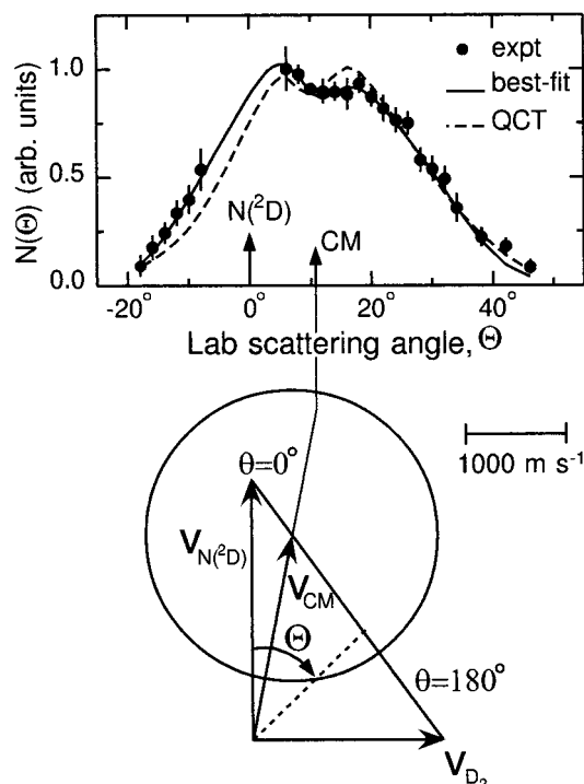
Figure 2. Laboratory ND angular distribution from the N(^2D) + D_2 reaction at E_c = 3.8 \text{ kcal mol}^{-1} and the corresponding Newton diagram showing the kinematics of the experiment. Solid line: calculated curve when using the best-fit CM angular and translational energy distributions. Dashed line: calculated curve when using the QCT derived CM angular and translational energy distributions.
