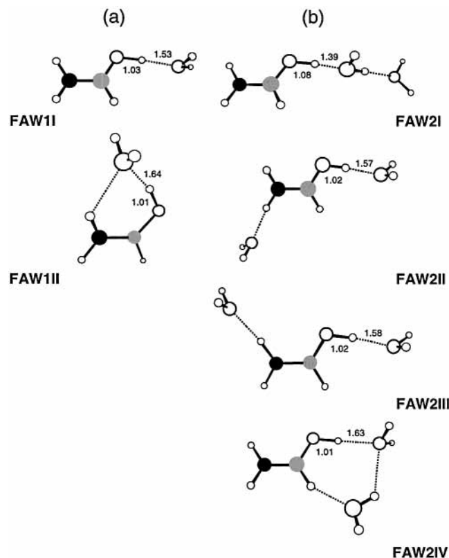
Figure 1. DFT-optimized structures of (a) \text{H}^+[\text{HC}(\text{O})\text{NH}_2](\text{H}_2\text{O}) and (b) \text{H}^+[\text{HC}(\text{O})\text{NH}_2](\text{H}_2\text{O})_2 . The C, N, O, and H atoms are denoted by shaded spheres, solid spheres, large open spheres, and small open spheres, respectively. The given bond lengths are all in the unit of angstrom.
