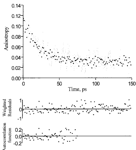
Figure 10. Example of simulation-based fit ( \bullet , \chi^2 = 1.01 ) of the experimental [\text{ZnM}(4\text{-Py})\text{TrPP}]_4 fluorescence anisotropy decay ( - ). \lambda_{\text{exc}} = 565\text{ nm} ; \lambda_{\text{det}} = 616\text{ nm} .
