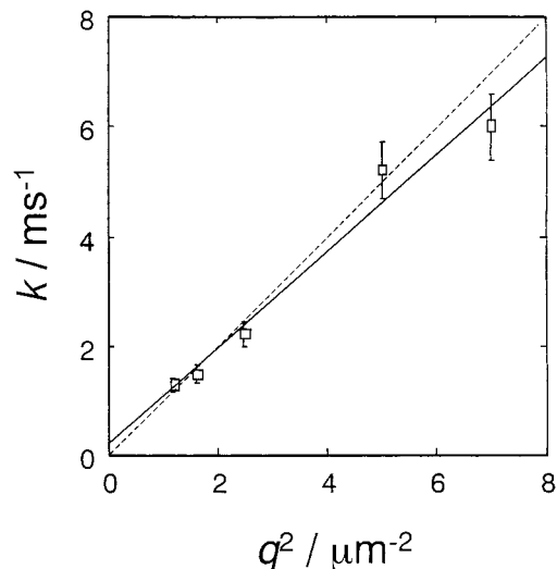
Figure 3. Relationship between the decay rate constants ( k ) of the TG signal of BQ •- and q^2 in water. The solid line is best-fitted line by the least-squares method. The dotted line is calculated k for BQ from D measured by the TD method.
