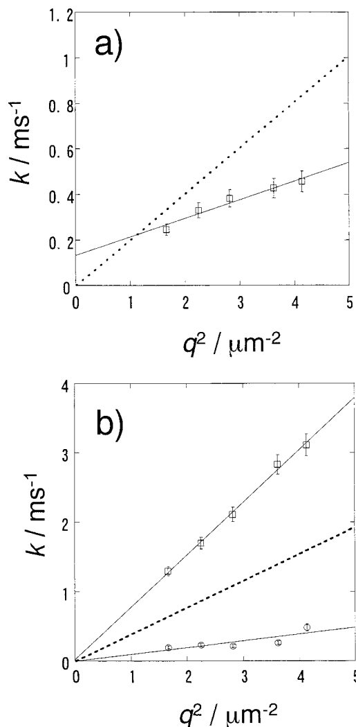
Figure 8. Relationship between the decay rate constants of the TG signal ( k ) of \text{AN}^{+\bullet} ( \square ) and q^2 (a) in the SDS and (b) in the CTAB solution. The solid line is the best-fitted line by the least-squares method. The dotted line is calculated k for AN from D measured by the TD method. Unknown component is also plotted ( \circ ).
