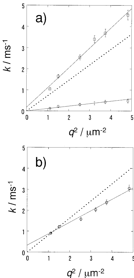
Figure 6. Relationship between the decay rate constants of the TG signal ( k ) of BQ •- (□) and q^2 (a) in the SDS and (b) in the CTAB solution (○). The solid line is the best-fitted line by the least-squares method. The dotted line is calculated k for BQ from D measured by the TD method. Unknown component is also plotted (○) in (a).
