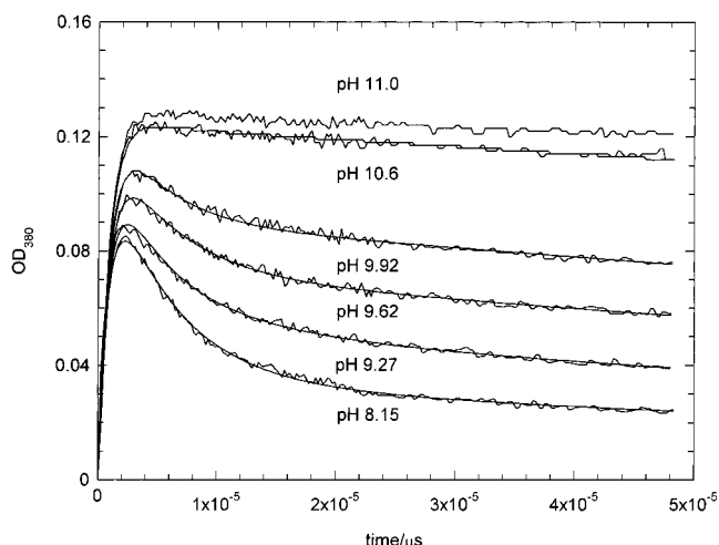
Figure 3. Absorbance at 380 nm as a function of time measured in 2 \times 10^{-4} M tellurite/hydrogen tellurite solutions at various pH values after irradiation (dose 19.8 Gy). The smooth curves are simulations calculated with the Gepasi package 21–23 (see text).
