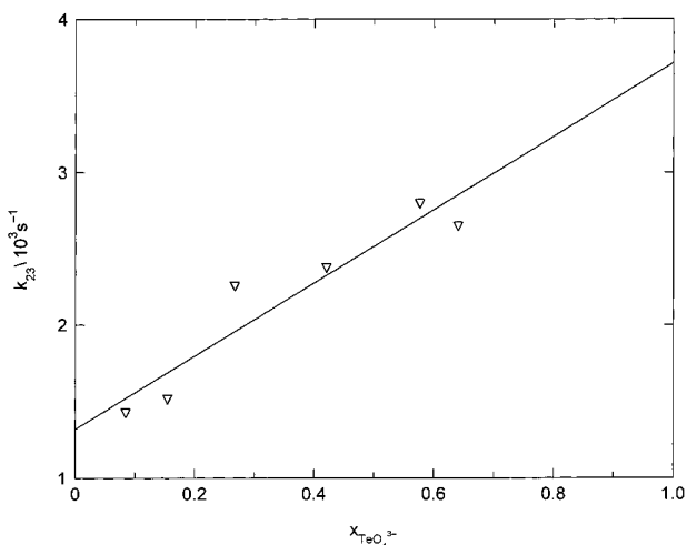
Figure 7. Determination of the rate constants k_{-4} and k_{-5} for the dissociation of \text{HTeO}_4^{2-} into \text{TeO}_3^{2-} and \text{OH}^- and the dissociation of \text{TeO}_4^{3-} into \text{TeO}_3^{2-} and \text{O}^- , respectively. k_{23} = k_{-5} \times \epsilon_{\text{TeO}_4^{3-}} \times x_{\text{TeO}_4^{3-}} + k_{-4} \times \epsilon_{\text{HTeO}_4^{2-}} \times (1 - x_{\text{TeO}_4^{3-}}) is plotted against x_{\text{TeO}_4^{3-}} \times x_{\text{TeO}_4^{3-}} is the fraction of \text{TeO}_4^{3-} present in the equilibrium mixture of \text{TeO}_4^{3-} and \text{HTeO}_4^{2-} . k_{23} is the first-order rate constant for the decay of absorbance at 325 nm. The straight line shows of a linear least-squares fit to the experimental points ( \times ).
