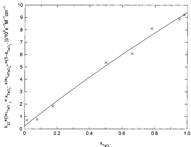
Figure 6. Determination of the second-order rate constants, k_{11} , k_{12} , and k_{13} , for the disappearance of \text{TeO}_3^- and \text{HTeO}_4^{2-} . k_{22} \times (x_{\text{TeO}_3^-} \times x_{\text{TeO}_3^-} + k_{\text{HTeO}_4^{2-}} \times (1 - x_{\text{TeO}_3^-})) is plotted against x_{\text{TeO}_3^-} . k_{22} is the rate constant of the second-order decay of absorbance at 350 nm (see text). x_{\text{TeO}_3^-} is the fraction of \text{TeO}_3^- present in the equilibrium mixture of \text{TeO}_3^- and \text{HTeO}_4^{2-} . Concentration of tellurite/hydrogen tellurite: 2 \times 10^{-4} M; dose 19.8 Gy; pH varies between 8 and 11. \times represents experimental points, the full line represents a least-squares fit of a quadratic function of x_{\text{TeO}_3^-} to the experimental points.
