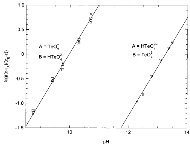
Figure 8. \text{p}K_{8,9} , the apparent acid dissociation constant of \text{TeO}_3^- , and \text{p}K_{10} , the acid dissociation constant of \text{HTeO}_4^{2-} , determined from plots of the quantity \log(\epsilon - \epsilon_A)/(\epsilon_B - \epsilon) against pH. In the left curve A and B stand for \text{TeO}_3^- and \text{HTeO}_4^{2-} , and in the right curve for \text{HTeO}_4^{2-} and \text{TeO}_4^{3-} , respectively. \Delta , \square , \times , and \nabla are experimental points, \Delta measured at 350 nm, \square at 400 nm, \times at 425 nm, and \nabla at 325 nm. Straight lines are linear least-squares fits to the experimental points.
