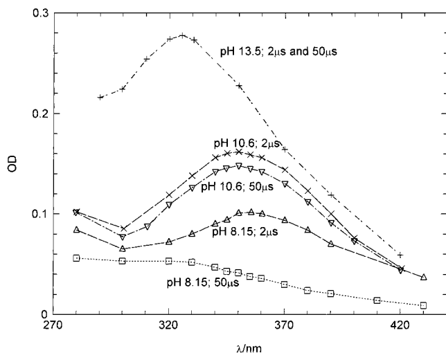
Figure 1. Transient absorption spectra measured 2 \mu\text{s} and 50 \mu\text{s} after irradiation (dose 19.8 Gy) of 2 \times 10^{-4} M tellurite/hydrogen tellurite solutions at pH 8.15, 10.6, and 13.5.
