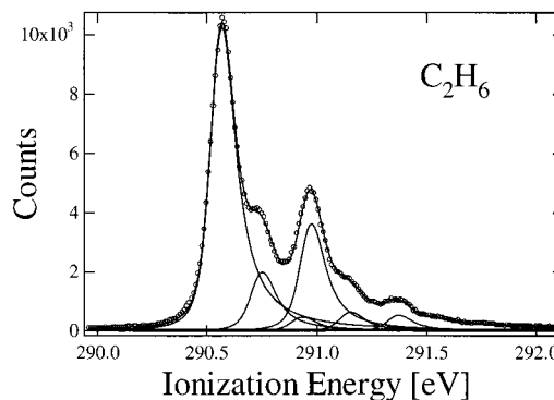
Figure 1. Carbon 1s photoelectron spectrum of ethane, as given by the circles, with an experimental resolution and lifetime broadening of 70 and 100 meV (fwhm), respectively. The solid line represents a free fit to the spectrum, as described in the text.
