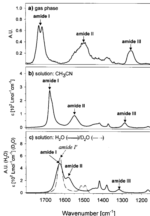
Figure 1. Experimental FTIR spectra in the amide I, II, and III region for N -methyl acetamide in (a) the gas phase, (b) acetonitrile solution, and (c) aqueous H 2 O (solid line) and D 2 O (dash-dot) solutions (c). The dipole strengths ( \mathbf{D} = 9.180 \times 10^{-3} \int \epsilon(\nu) d\nu/\nu_{\max} ) are as follows: for acetonitrile, \mathbf{D}(\text{amide I}) = 5.2 \times 10^{-2} \text{ D}^2 , \mathbf{D}(\text{amide II}) = 2.6 \times 10^{-2} \text{ D}^2 ; for D 2 O, \mathbf{D}(\text{amide I}') = 11.1 \times 10^{-2} \text{ D}^2 . Concentrations were 190 mM (acetonitrile) and 137 mM (D 2 O).
