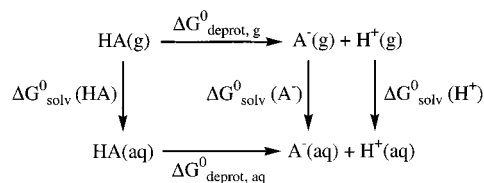
Figure 2. Thermodynamic cycle used in the calculation of pK_a . 17,18
