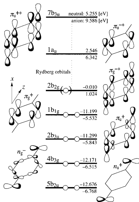
Figure 1. Some important Hartree–Fock molecular orbitals and their energies of p -BQ and its anion radical. The molecular axes are shown in the figure. Subscripts g and u stand for the symmetry for the inversion center, and superscripts + and - stand for the symmetry for the xy plane of the molecule. LUMO of neutral p -BQ (2b 2g ; \pi_g^{-*} ) is to be SOMO for the anion radical.
