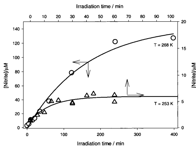
Figure 2. Nitrite concentration as a function of irradiation time in ice pellets made of 10 mM NaNO 3 aqueous solutions: (Δ) at 253 K; (O) at 268 K.
