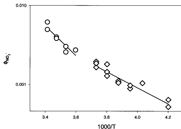
Figure 6. Quantum yields of nitrite formation \phi_{\text{NO}_2^-} vs 1000/T (in kelvins) in 10 mM \text{NaNO}_3 aqueous solutions (O) and in ice pellets made of the same solutions ( \diamond ).
