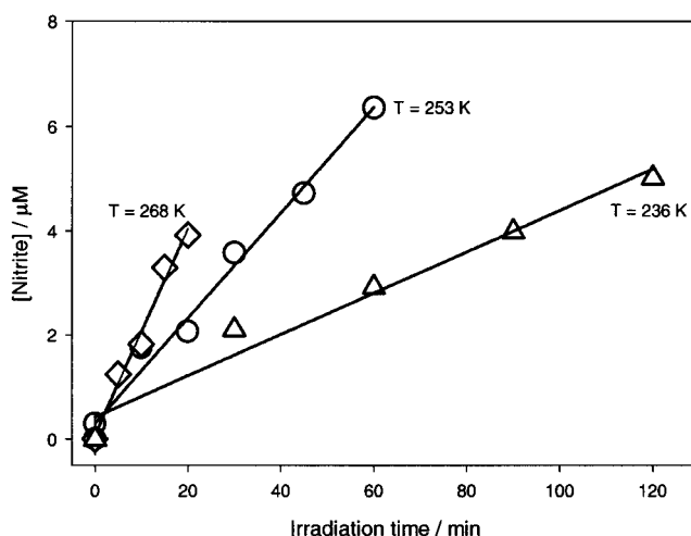
Figure 3. Nitrite concentration as a function of irradiation time in ice pellets made of 1 mM NaNO 3 + 10 mM NaCO 2 H aqueous solutions at different temperatures: (Δ) 236 K; (O) 253 K; (◇) 268 K.
