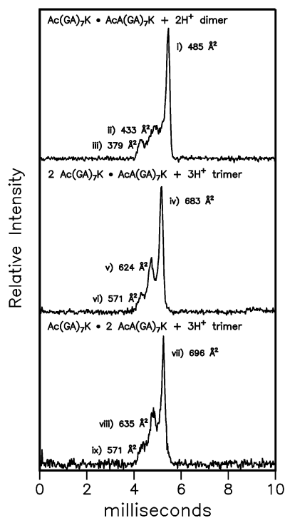
Figure 2. Drift time distributions recorded for the dimer and trimer ions obtained from the \text{Ac}-(\text{GA})_7\text{K} and \text{Ac}-\text{A}(\text{GA})_7\text{K} mixture. The main features in the drift time distributions are labeled i–ix for reference and assigned cross sections.
