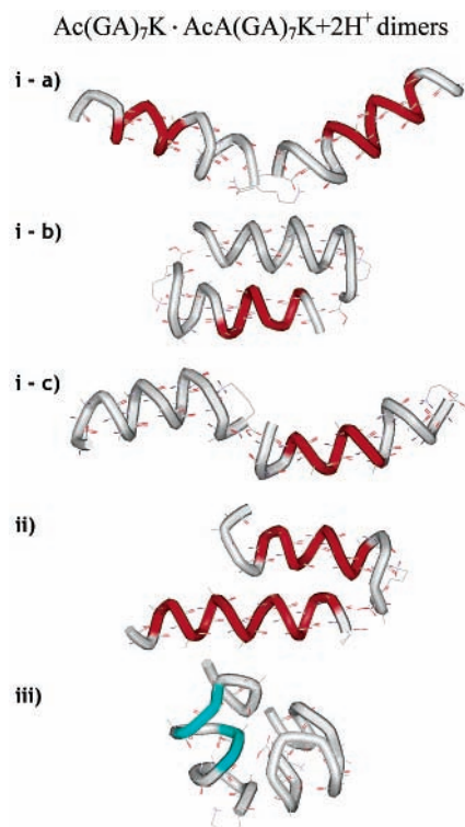
Figure 6. Ac-(GA) 7 K·Ac-A(GA) 7 K+2H + dimer conformations obtained from MD simulations. The labels refer to possible assignments to the features in the measured drift time distribution (Figure 2). The images were produced using the WebLab viewer (Molecular Simulations Inc., San Diego, CA). The red regions are \alpha helix, and the blue regions are \beta sheet.
