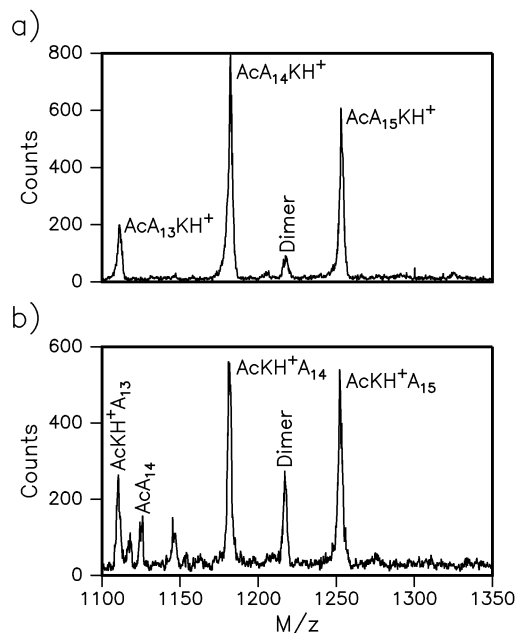
Figure 4. Electrospray mass spectra recorded for mixtures of (a) \text{Ac}-\text{A}_{14}\text{K} and \text{Ac}-\text{A}_{15}\text{K} and (b) \text{Ac}-\text{KA}_{14} and \text{Ac}-\text{KA}_{15} in 90% TFA/10% water.
