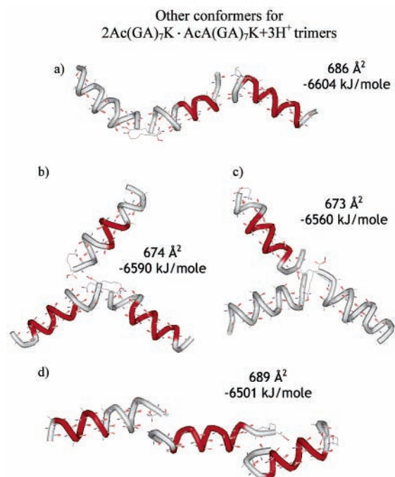
Figure 8. Other conformations which match the cross section for the dominant feature in the drift time distribution of the 2Ac-(GA) 7 K·Ac-A(GA) 7 K+3H + trimer, Figure 2iv. The images were produced using the WebLab viewer (Molecular Simulations Inc., San Diego, CA). The red regions are \alpha helix, and the blue regions are \beta sheet.
