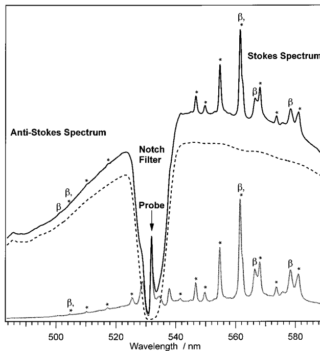
Figure 1. Representative pump + probe (solid-line), pump-only (dashed line), and probe-only (dotted line) spectra of \beta -carotene. The pump + probe time delay is 1 ps. The dip in the middle of the spectrum is due to the notch filter, which removes scattered light within 5 nm of the probe wavelength (visible as the peak in the middle of the notch). Pump-induced fluorescence from \text{S}_2 spans the entire spectral window. Peaks labeled with an asterisk (*) are due to toluene. Peaks due to \beta -carotene are labeled " \beta ".
