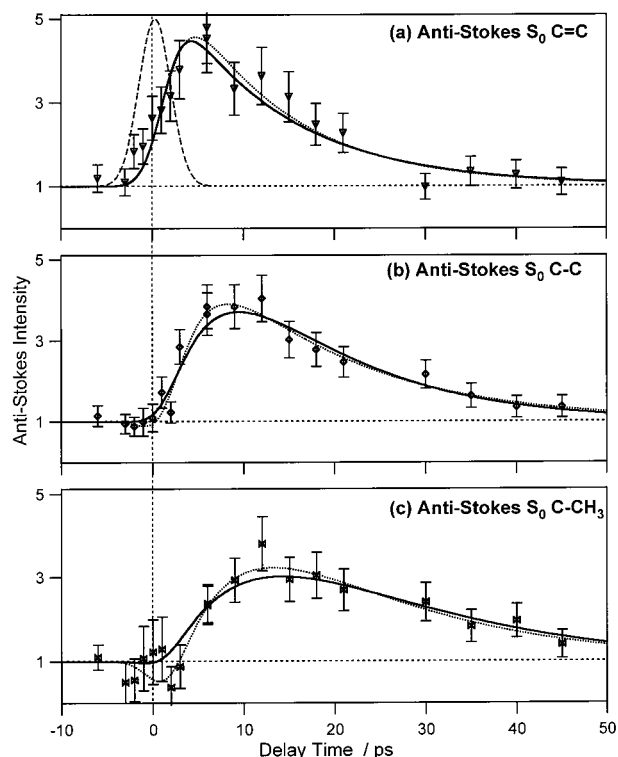
Figure 6. Kinetics of the time-resolved anti-Stokes \beta -carotene spectra. Data points are the integrated areas of the anti-Stokes S_0 C=C peak at 1523 cm -1 (a), the S_0 C-C peak at 1157 cm -1 (b) and the S_0 C-CH 3 peak at 1004 cm -1 (c). The 4.1 ps fwhm Gaussian instrumental response is shown as the dashed curve in (a). The other curves are the best-fit convolutions of the instrument response with either a biexponential (eq 1, dotted) or kinetic (eq 8, solid) model of the molecular response. Values of the best fit parameters are summarized in Tables 1 and 2. Each peak area has been normalized to its area in the probe-only spectrum.
