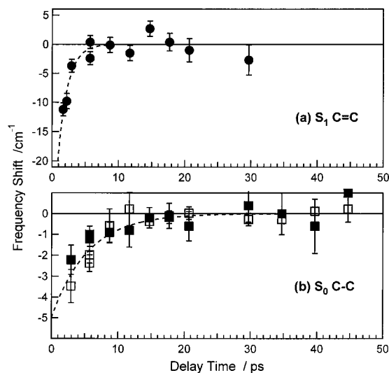
Figure 7. Time-dependent frequency shifts of the S_1 C=C and S_0 C-C Raman peaks of \beta -carotene. (a) The frequency of the Stokes S_1 C=C mode relative to 1781 cm -1 . The dashed line is a 1.4 ps exponential decay. (b) The frequency shifts of the Stokes (open squares) and anti-Stokes (filled squares) S_0 C-C peaks relative to 1157 cm -1 . The dashed line is a 5.4 ps exponential decay, determined by the anti-Stokes C-C kinetics.
