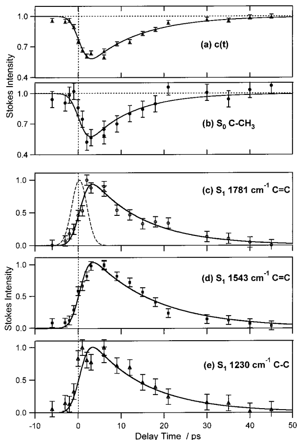
Figure 5. Kinetics of the time-resolved Stokes spectra of \beta -carotene. The top two panels present the dynamics of S_0 population depletion and recovery. The subtraction coefficient, c(t) , was used to scale the probe-only spectrum in the generation of the Stokes difference spectra. The S_0 C-CH 3 intensity (b) is the integrated area of the methyl-rock peak at 1004 cm -1 in the pump + probe spectra. The bottom three panels present the dynamics of the S_1 state monitored by the Stokes difference spectra. The data points are the integrated areas of the S_1 C=C peak at 1781 cm -1 (c), the C=C band at 1543 cm -1 (d), and the C-C band at 1230 cm -1 (e). The 4.1 ps fwhm Gaussian instrumental response is shown as the dashed curve in (c). The solid curves are the fits of a convolution of the instrument response with the exponential molecular response described in eq 1. The fitting parameters are summarized in Table 1.
