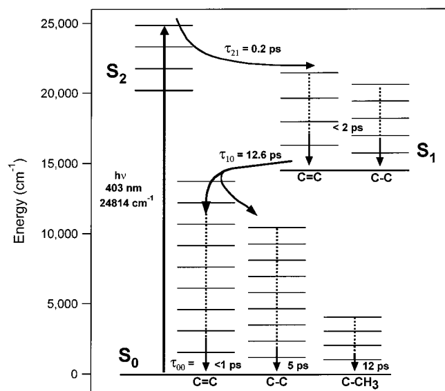
Figure 8. Vibronic relaxation scheme of \beta -carotene. After excitation to S_2 ( 1B_u^+ ), the molecule relaxes in 0.2 ps to S_1 ( 2A_g^- ). In S_1 IVR occurs very rapidly, such that the population of vibrational states with \nu = 1 is less than 10% within 2 ps. Internal conversion from S_1 to S_0 ( 1A_g^- ) occurs with a 12.6 ps time constant. The C=C mode is the primary accepting mode of the IC process and relaxes in <1 ps through IVR. The C-C mode is excited directly by IC, as a minor accepting mode, and relaxes with a \sim 5 ps time constant. The C-CH 3 mode is excited by the IVR process and then relaxes with a \sim 12 ps time constant, which is likely the molecular cooling rate.
