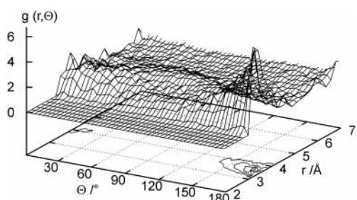
Figure 11. Exemplary angle-dependent RDF g_{C(1)-C(2),C(1)-C(2)}(r) of the 11.6 mol % AN mixture.
