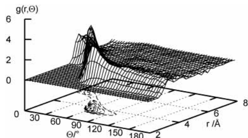
Figure 6. Angular-dependent RDF g_{N-C(2),N}(r, \Theta) of the 11.6 mol % AN mixture. The correlated atom pairs are the nitrogen atoms of the AN molecules. The contour lines display the angular and radial positions of the local maxima.
