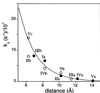
Figure 6. Exponential dependence of the quenching rate constants with the distance in deuterated water. Closed circles, monodeprotonated species; open circles, dideprotonated (and triprotonated) species.
