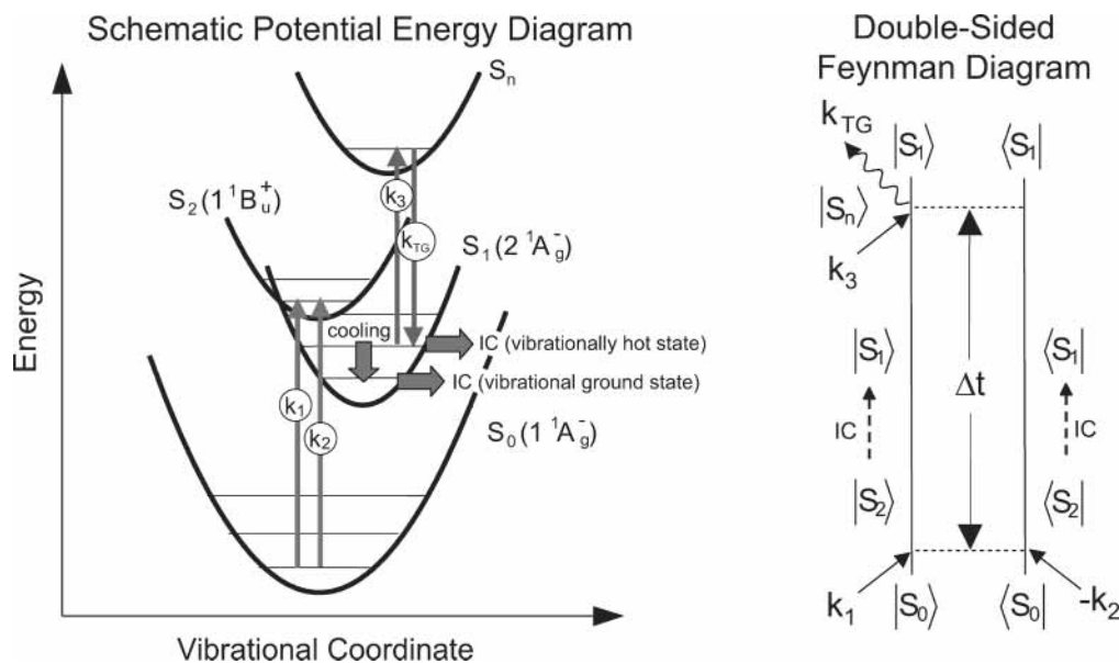
Figure 1. Schematic Potential Energy Diagram of \beta -carotene (left) and the double-sided Feynman diagram (right) illustrating the transient grating technique used to determine the kinetics of the S_1/S_0 internal conversion initiating out of vibrationally excited as well as ground state modes. Two pump lasers ( 1 and 2 , \lambda_{\text{pu}} = 510 nm, fwhm = 70 fs, 60 nJ), induce a population grating of electronically excited molecules in the S_2 state of \beta -carotene. The subsequent S_2/S_1 internal conversion populates the S_1 state that is probed by elastically scattering a third probe pulse ( 3 , \lambda_{\text{pu}} = 570 –660 nm, fwhm = 70 fs, 60 nJ) off the population grating, generating the coherent signal 4 ( k_{\text{TG}} ) in the phase-matched direction. The probe pulse is delayed variably in time ( \Delta t ) relative to the two laser pump pulses that interact simultaneously with the sample to induce the population grating. The probe pulse is tuned variably to be in resonance to the S_n \leftarrow S_1 optical transition and furthermore spectrally red-shifted out of this optical transition to enhance the interrogation of vibrationally excited states in the S_1 potential.
