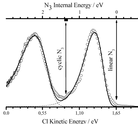
Figure 3. The translational energy distribution for ground-state Cl ( ^2P_{3/2} ) derived from the velocity map image shown in Figure 2. The arrow at E_{kin} = 1.65 eV marks the maximum possible translational energy to form Cl with linear- N_3 ( \tilde{X}\ ^2\Pi ). The double-headed arrow marked “cyclic- N_3 ” shows where a new feature of the Cl atom energy spectrum appears reflecting formation of an excited form of N_3 . The most recent theoretical predictions of the cyclization energy of N_3 are shown as the black bar.
