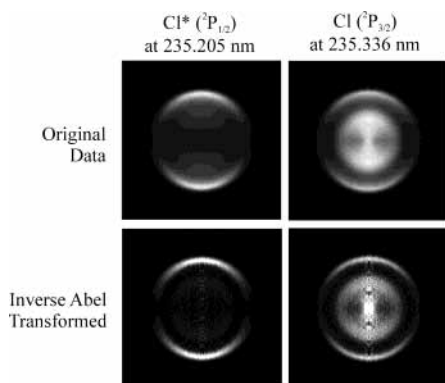
Figure 2. Raw and inverse Abel transformed images of Cl ( ^2P_{3/2} ) recorded with dissociation and probe at \lambda = 235.336 nm on the 4p\ ^2D_{3/2} \leftarrow 2p\ ^2P_{3/2} transition and of Cl* ( ^2P_{1/2} ) recorded with dissociation and probe at \lambda = 235.205 nm on the 4p\ ^2P_{1/2} \leftarrow 2p\ ^2P_{1/2} transition. The laser polarization direction is vertical in the plane of the images.
