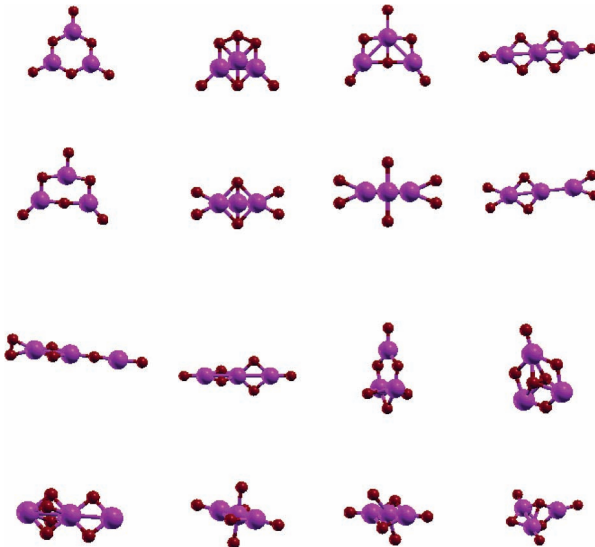
Figure 1. Schematic representation of different isomers considered in this study for \text{Al}_3\text{O}_6 . Aluminum and oxygen atoms are represented by large and small filled circles, respectively.
