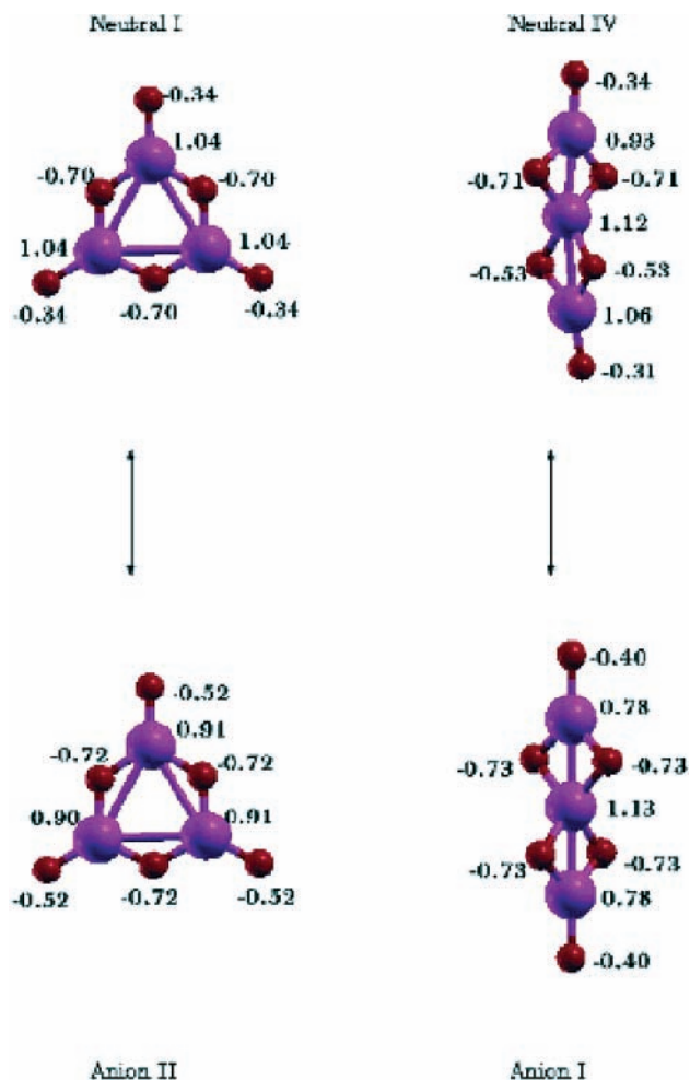
Figure 5. Schematic representation of Mulliken charges in neutral and anionic Al 3 O 6 .
