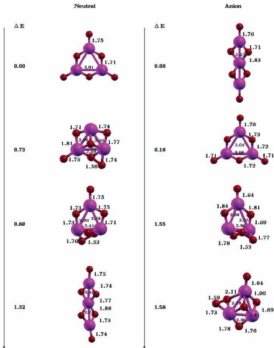
Figure 2. Some of the lowest energy configurations of neutral and anionic \text{Al}_3\text{O}_6 . Energy difference is in eV. Aluminum and oxygen atoms are represented by large and small filled circles, respectively.
