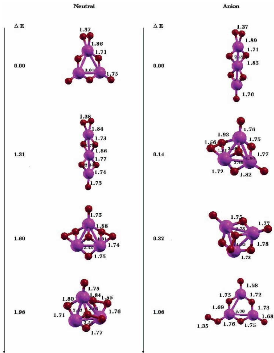
Figure 3. Some of the lowest energy configurations of neutral and anionic \text{Al}_3\text{O}_7 . Energy difference is in eV. Aluminum and oxygen atoms are represented by large and small filled circles, respectively.
