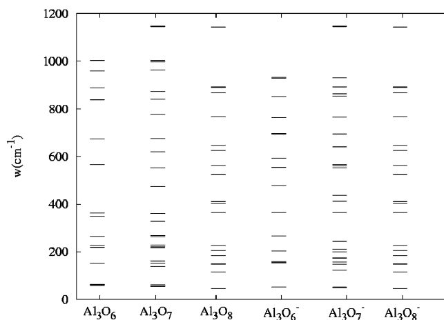
Figure 6. Vibrational frequency spectra of neutral and anionic Al 3 O n ( n = 6-8 ).
