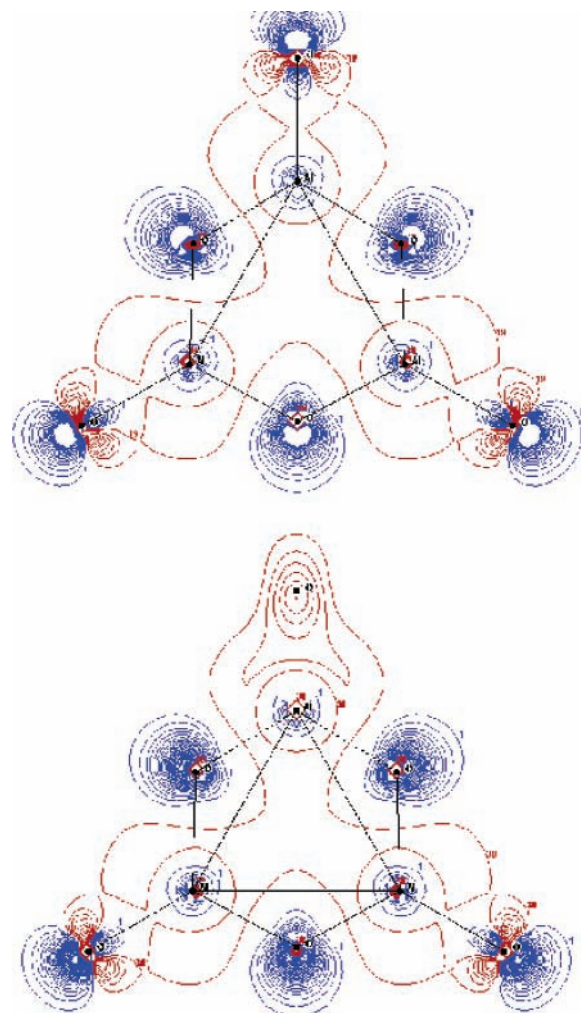
Figure 7. Difference charge-density, \Delta\rho , surfaces for the lowest energy structure of \text{Al}_3\text{O}_6 (upper) and \text{Al}_3\text{O}_7 (lower). The charge densities have been given for 0.01 electron/au respectively.
