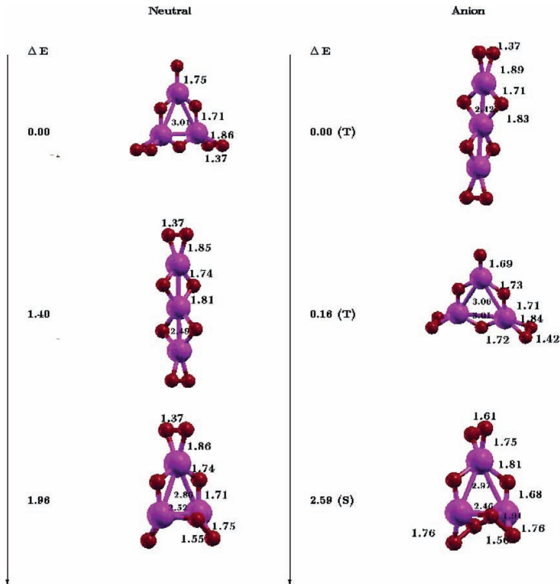
Figure 4. Some of the lowest energy configurations of neutral and anionic \text{Al}_3\text{O}_8 . Energy difference is in eV. Aluminum and oxygen atoms are represented by large and small filled circles, respectively.
