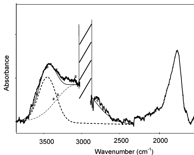
Figure 2. IR spectrum of \text{H}_5\text{O}_2^+ triflate in DCE showing deconvolution of \nu\text{O}-\text{H} .
