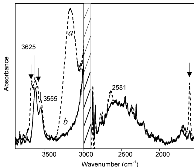
Figure 4. IR spectrum of 0.01 M (\text{CF}_3\text{SO}_2)_2\text{NH} containing 0.01 M \text{H}_2\text{O} in DCE before (a) and after (b) subtraction of the spectra of free acid and free dissolved water molecules (marked by arrows). Spectrum b (solid line) belongs primarily to the dihydrated acid.
