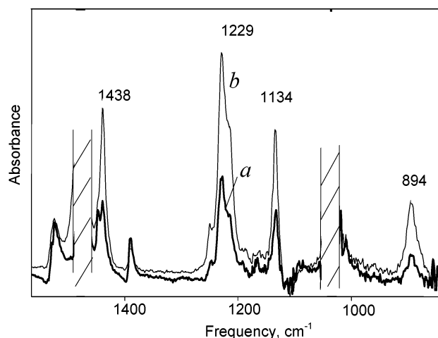
Figure 5. IR spectra of complexes (a) \text{H}_2\text{O}\cdot\text{HN}(\text{SO}_2\text{CF}_3)_2 7 and (b) \text{H}_2\text{O}\cdot\text{H}_2\text{O}\cdot\text{HN}(\text{SO}_2\text{CF}_3)_2 8 in benzene solution in the frequency range of anion vibrations.
