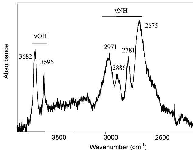
Figure 3. Spectrum of (CF 3 SO 2 ) 2 NH·OH 2 in CCl 4 derived from the spectrum of 0.01 M HN(SO 2 CF 3 ) 2 solution containing 0.0036 M water after subtraction of the spectra of free water and anhydrous acid. The very broad νN–H band is split into several bands by Fermi resonance effects.
