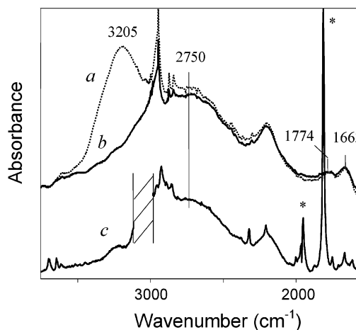
Figure 1. IR spectra of DCE solutions of 0.0225 M triflic acid containing 0.0075 M H 2 O before (a) and after (b) subtraction of the remaining free acid. Spectrum c was obtained in the same way from IR spectra of benzene solution of 0.0667 M triflic acid + 0.01 M H 2 O. Both spectra b and c belong to [H 3 O][CF 3 SO 3 ]. Nonsubtracted bands of benzene that form a \pi -complex are marked with an asterisk.
