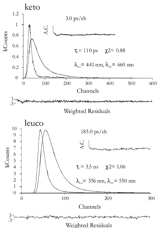
Figure 3. Fluorescence decays and pulse instrumental response obtained for the keto and leuco forms of indigocarmine in DMF at T = 293 K. The experimental conditions and obtained decay times are shown as insets in the figure. Also shown are the weighted residuals, autocorrelation functions (A.C.) and the \chi^2 values for a better judgment of the quality of the fits.
