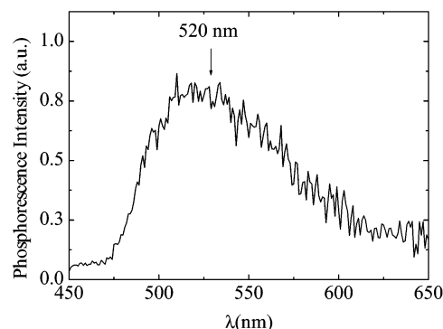
Figure 4. Phosphorescence spectra of the leuco form of indigocarmine in methanol at T = 77 K (a few drops of the sodium dithionite/NaOH aqueous solution were added to induce the formation of the leuco form).
