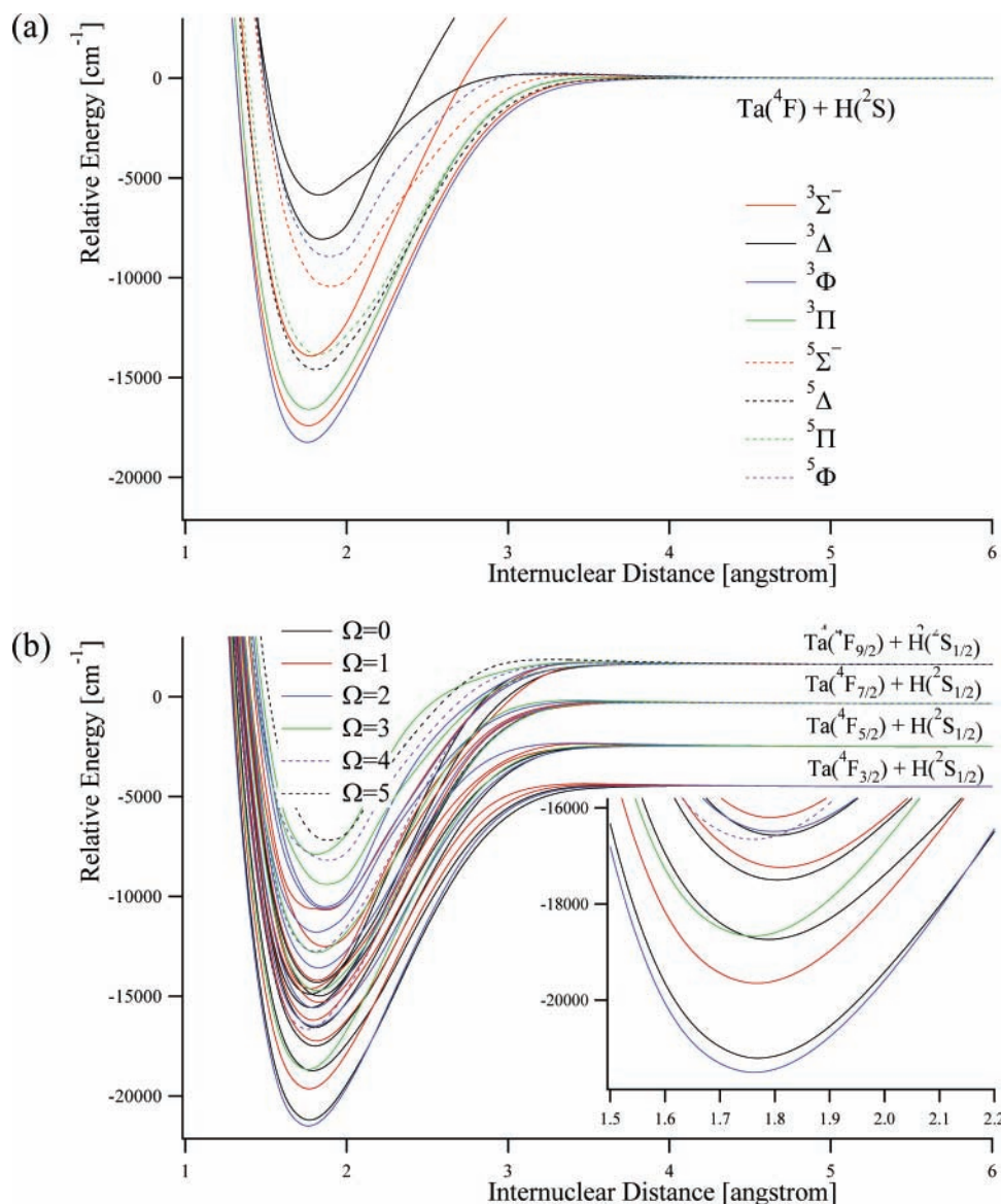
Figure 3. TaH potential energy curves obtained with use of triplet MCSCF+SOC/ SBKJC(f,p) wave functions: (a) low-lying adiabatic states and (b) low-lying spin-mixed states. The inset figure is a close-up view near the energy minima.
