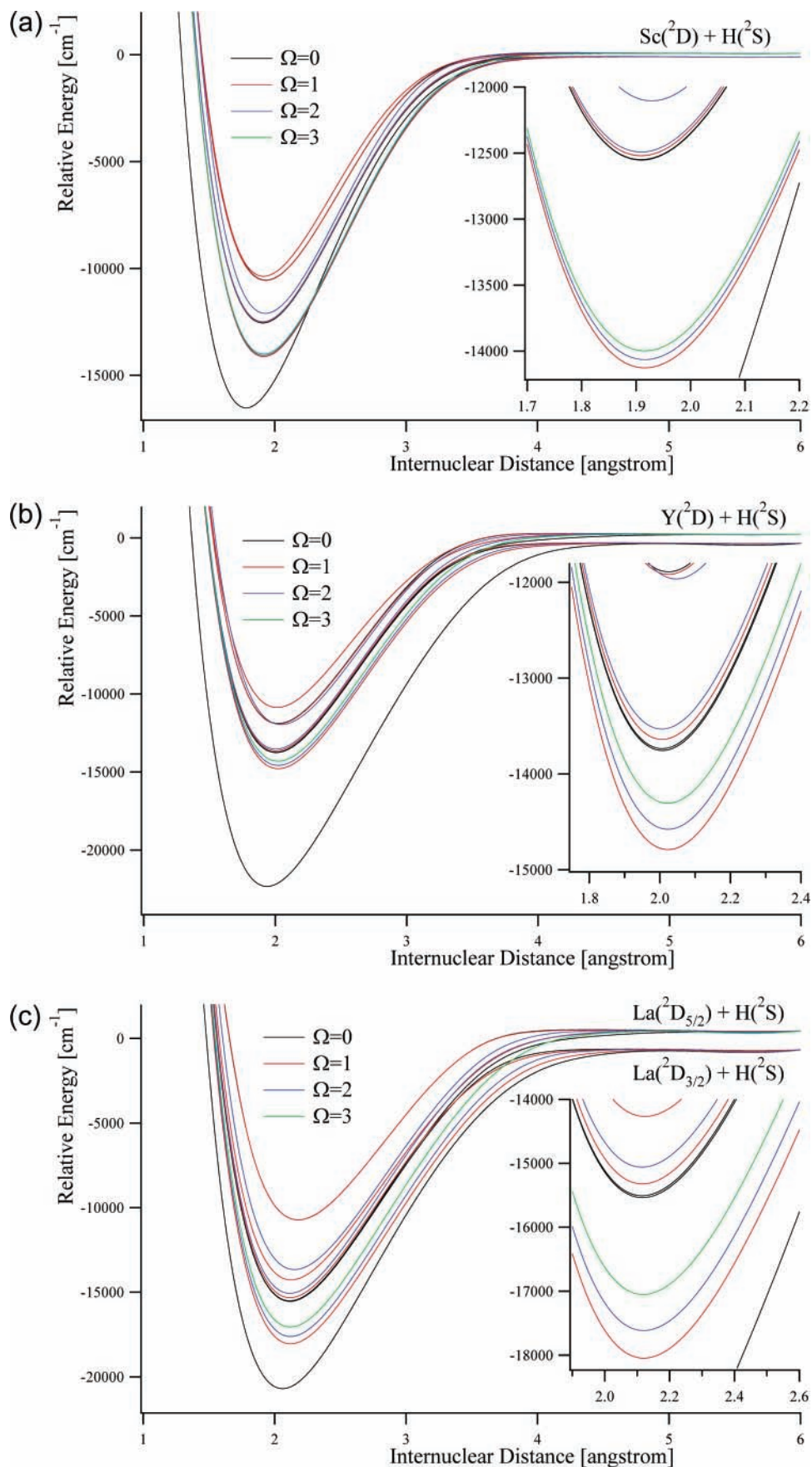
Figure 4. Potential energy curves of low-lying spin-mixed states obtained with use of singlet MCSCF+SOC/ SBKJC(f,p) wave functions: (a) ScH, (b) YH, and (c) LaH. The inset figures are close-up views near the energy minima.
