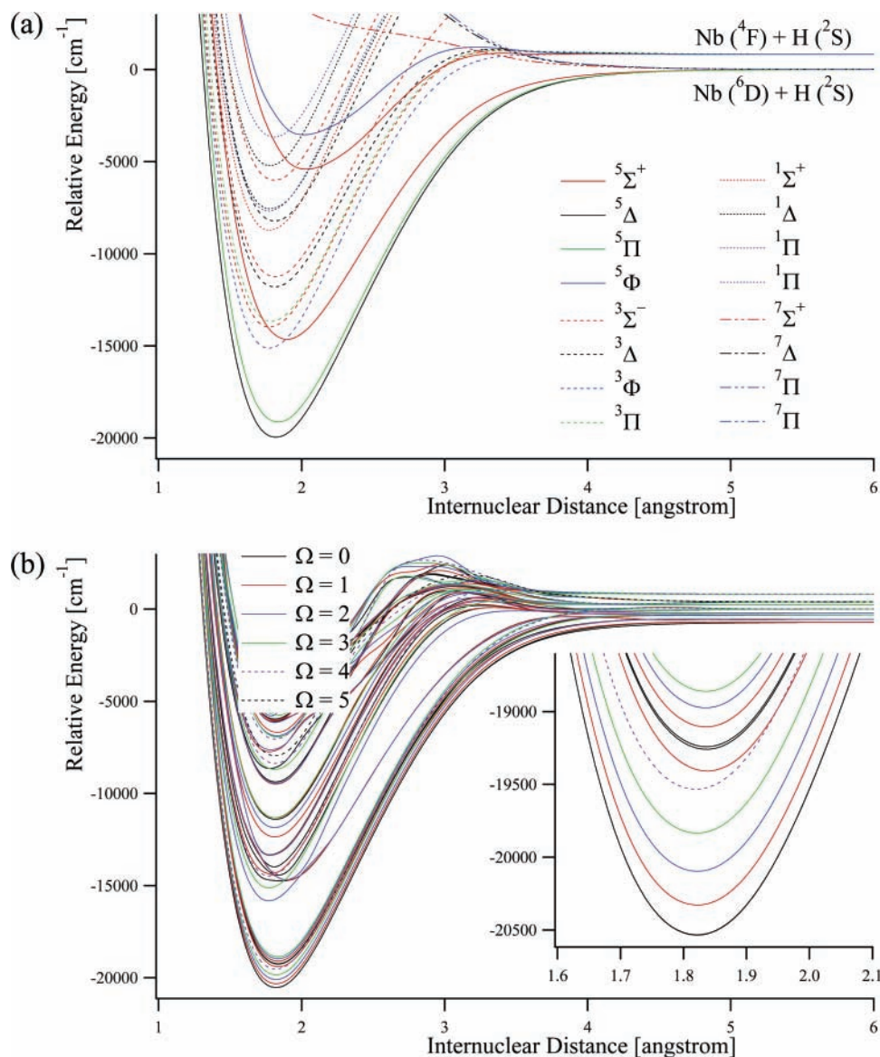
Figure 2. NbH potential energy curves obtained with use of quartet MCSCF+SOC1/SBKJC(f,p) wave functions, where the MCSCF active space includes two sets of 4d and 5s orbitals: (a) low-lying adiabatic states and (b) low-lying spin-mixed states. The inset figure is a close-up view near the energy minima.
