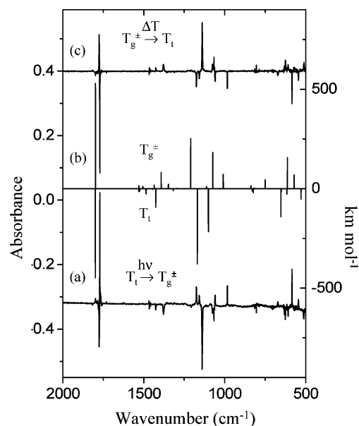
Figure 5. Difference IR absorption spectra for PA-OH showing (a) the effect of excitation of the 2\nu\text{OH} mode of the monomer isolated in an Ar matrix, (b) the MP2/6-311G(2d,2p) calculated spectra for the T_1 (negative bands) and T_g^\pm (positive bands) forms of propionic acid, and (c) the effect of annealing an Ar matrix containing the T_1 and T_g^\pm conformers at 12 K for \sim 20 min.
