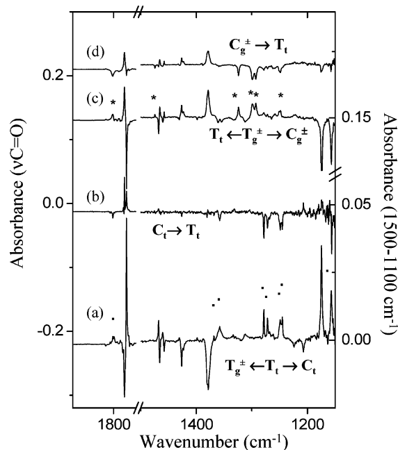
Figure 4. Spectral changes upon excitation of the 2\nu\text{OH} mode of T_1 and T_g^\pm conformers (traces a and c, respectively) and dark decay of the C_t (■) and C_g^\pm (*) conformers (traces b and d, respectively). Difference spectra a and c are obtained by subtracting the spectra recorded before pumping from those recorded under pumping. Difference spectra b and d are obtained by subtracting the spectra recorded under pumping from those recorded after a few minutes in the dark.
