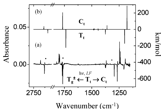
Figure 6. Difference IR absorption spectra for PA-OD showing (a) the result of vibrational excitation of the T_t conformer at 5170\text{ cm}^{-1} (LF) and (b) the MP2/6-311++(2d,2p) calculated spectra for the T_t (negative bands) and C_t (positive bands) forms. In plot a, the bands of the C_t and T_g^\pm (marked with dots) conformers increase, and the T_t bands decrease.
