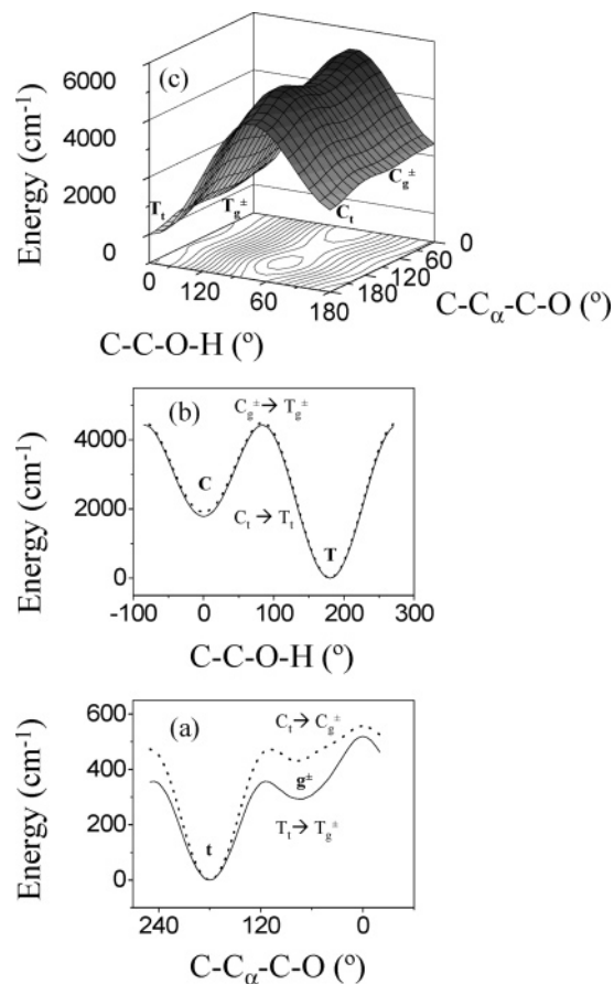
Figure 2. One- and two-dimensional potential energy surfaces (PES) of propionic acid as a function of the C α -C and C-O torsional coordinates. (a) Rotation along the C α -C axis, which corresponds to the T t ↔ T g ± (solid line) and C t ↔ C g ± (dotted line) isomerization reactions. (b) Rotation along the C-O axis, which corresponds to the T t ↔ C t (solid line) and T g ± ↔ C g ± (dotted line) isomerization reactions. (c) Simultaneous rotation along the C α -C and C-O axes. The lowest-energy minimum is set to zero.
