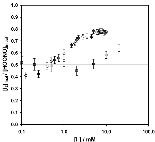
Figure 5. Relative yields of diiodine from the oxidation of iodide by peroxyntrous acid vs total iodide concentration: 0.1 M phosphoric acid/phosphate buffers.; circles, [\text{HOONO}]_{\text{initial}} = 25 \mu\text{M} ; squares, [\text{HOONO}]_{\text{initial}} = 5 \mu\text{M} .
