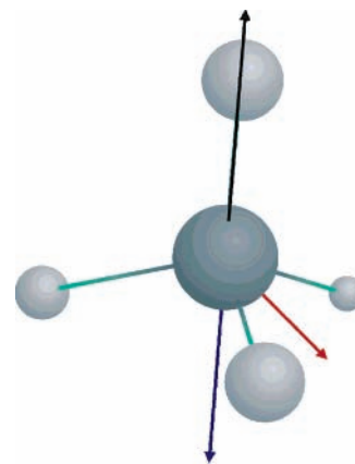
Figure 2. Directions into which potential curves for electron emission are calculated for the tetrahedral anions \text{XO}_4^{2-\beta-} with X = \text{S, Se, As, and P} . Color code: threefold axis, X–O (positive direction), black; threefold axis, O–X (negative direction), blue; twofold axis, O–Y ( Y is the midpoint between two oxygen atoms), red.
