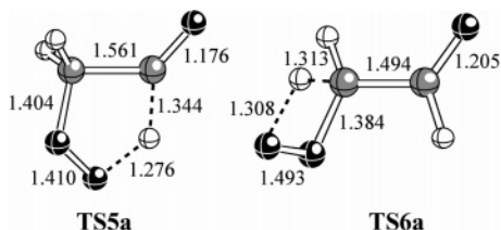
Figure 7. Transition structures for intramolecular hydrogen shifts in the 2-oxoethylperoxy radical. Bond lengths (in Å) computed at the B3LYP/6-311G(2d,d,p) level.
