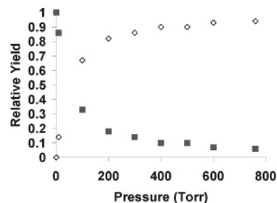
Figure 12. Relative yields of thermalized 1-oxo-2-propylperoxy radical 4c ( \diamond ) and 2-hydroperoxypropanoyl radical 8c ( \blacksquare ) predicted by master equation simulations.
