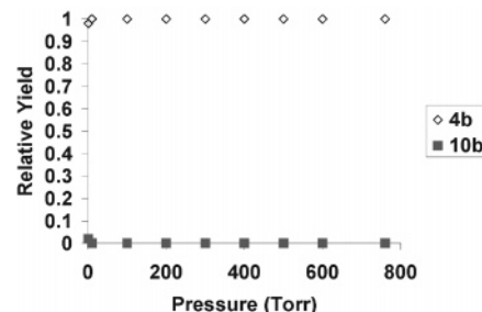
Figure 11. Relative yields of thermalized acetylperoxy radical 4b ( \diamond ) and 3-hydroperoxyacetyl radical 10b ( \blacksquare ) predicted by master equation simulations.
