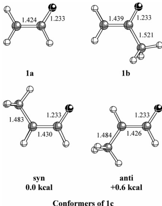
Figure 1. Structures of the parent ( 1a ) and methyl-substituted ( 1b and 1c ) vinyloxy radicals. Bond lengths (in Å) computed at the B3LYP/6-311G(2d,d,p) level, and relative energies (in kcal/mol) computed with the CBS-QB3 method. Note that in all figures, gray represents carbons, white represents hydrogens, and black represents oxygens.
