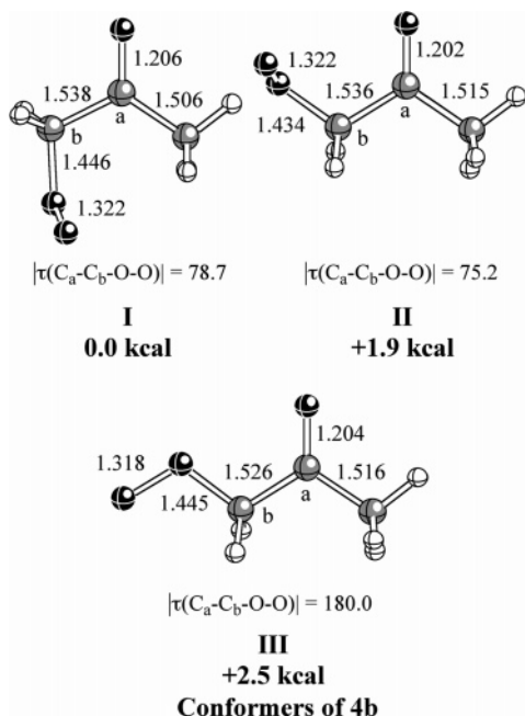
Figure 5. Structures of the 2-oxo-1-propylperoxy (or acetylperoxy) radical. Bond lengths (in Å) and torsional angles (in degrees) computed at the B3LYP/6-311G(2d,d,p) level, and relative energies (in kcal/mol) computed with the CBS-QB3 method.
