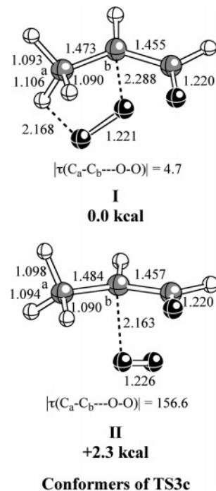
Figure 3. Transition structures for the addition of O 2 to 2-methylvinyloxy radical ( TS3c ). Bond lengths (in Å) and torsional angles (in degrees) computed at the B3LYP/6-311G(2d,d,p) level, and relative energies (in kcal/mol) computed with the CBS-QB3 method.
