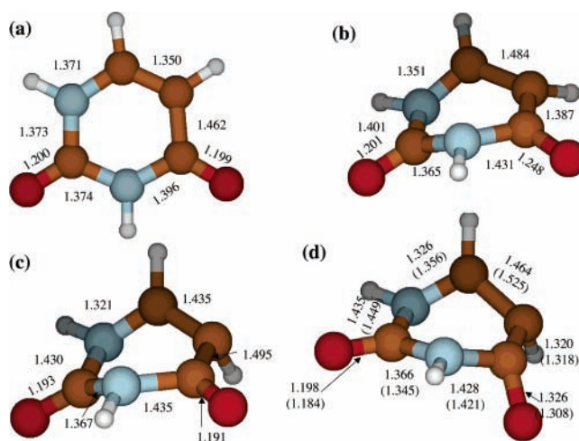
Figure 2. Geometry of uracil at (a) the S_0 minimum, (b) the S_1-S_2 conical intersection, (c) the S_0-S_1 conical intersection, and (d) the three-state S_0-S_1-S_2 conical intersection. All bond distances between non-hydrogen atoms are shown in Å. MRCII results are shown, except in (d), where the MRCI \sigma results are also shown in parentheses. More internal coordinates are given as Supporting Information.
