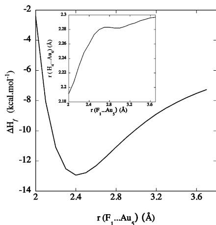
Figure 8. Section of the PES of \text{Au}_3-(\text{HF})_2 as a function of r(\text{F}_1 \cdots \text{Au}_5) \in [2.0 \text{ \AA}, 3.7 \text{ \AA}] relative to the total energy of monomers. The insert depicts the optimized H-bond length r(\text{H}_4 \cdots \text{Au}_6) as a function of r(\text{F}_1 \cdots \text{Au}_5) \in [2.0 \text{ \AA}, 3.7 \text{ \AA}] .
