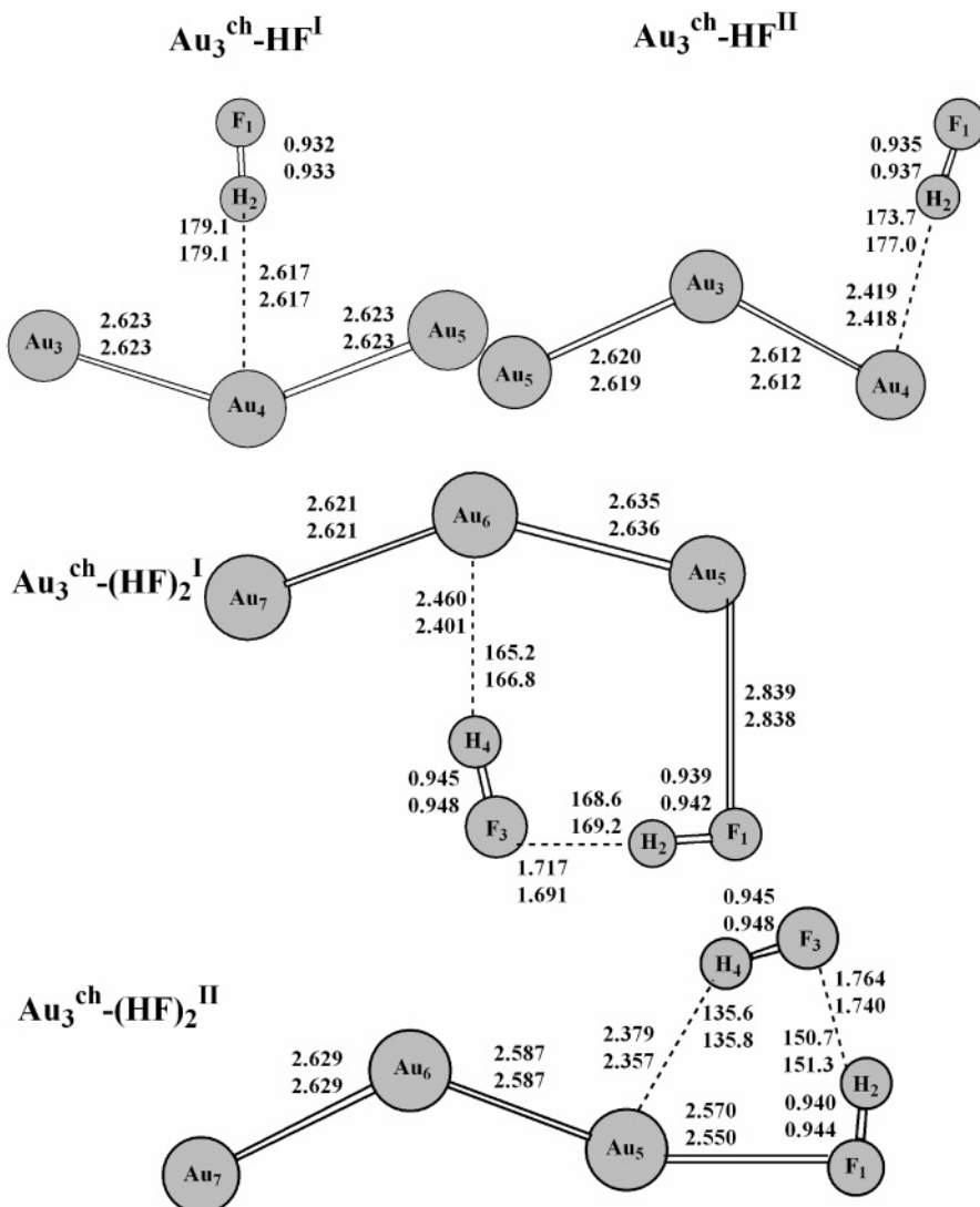
Figure 2. Lower-energy complexes of \text{Au}_3^{\text{ch}}\text{-(HF)} and \text{Au}_3^{\text{ch}}\text{-(HF)}_2 obtained within the B3LYP/RECP(Au)UA(H,F) (top entry) and B3LYP/RECP(Au)UB(H,F) (lower entry) approaches. Some selected properties of these complexes relevant for a further discussion are collected in Table 1. The bond lengths are given in Å and bond angles in deg. In addition, the values of some bond angles of the structures \text{Au}_3^{\text{ch}}\text{-(HF)}_2^{\text{I}} : \angle\text{Au}_5\text{F}_1\text{H}_2 = 88.6^\circ\text{A} , 88.1^\circ\text{B} , \angle\text{H}_2\text{F}_3\text{H}_4 = 110.8^\circ\text{A} , 110.1^\circ\text{B} ; and \text{Au}_3^{\text{ch}}\text{-(HF)}_2^{\text{II}} : \angle\text{Au}_5\text{F}_1\text{H}_2 = 93.1^\circ\text{A} , 92.8^\circ\text{B} , \angle\text{H}_2\text{F}_3\text{H}_4 = 94.5^\circ\text{A} , 94.1^\circ\text{B} .
