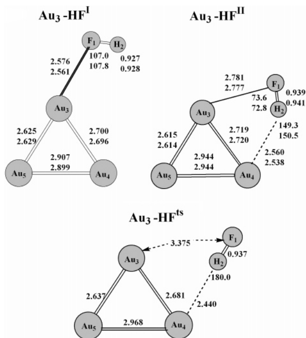
Figure 1. Lower-energy complexes of \text{Au}_3\text{-HF} obtained within the B3LYP/RECP(Au)UA(H,F) (top entry) and B3LYP/RECP(Au)UB(H,F) (lower entry) approaches. Some selected properties of these complexes relevant for a further discussion are collected in Table 1. The complex \text{Au}_3\text{-HF}^{\text{I}} is almost twice as polar (2.6–2.8 D) as the \text{Au}_3\text{-HF}^{\text{II}} one (1.4–1.5 D). The transition-state structure \text{Au}_3\text{-HF}^{\text{ts}} is identified within the B3LYP/RECP(Au)UA(H,F) approach. The bond lengths are given in Å and bond angles in deg.
