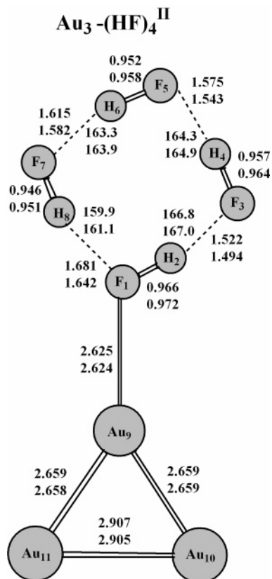
Figure 7. \text{Au}_3-(\text{HF})_4^{\text{II}} complex obtained within the B3LYP/RECP-(Au)U(A)(H,F) (top entry) and B3LYP/RECP(Au)U(B)(H,F) (lower entry) approaches. Its selected properties relevant for a further discussion are collected in Table 1. The bond lengths are given in Å and bond angles in deg. In addition, the values of some bond angles of \text{Au}_3-(\text{HF})_4^{\text{II}} : \angle\text{H}_2\text{F}_3\text{H}_4 = 106.6^\circ\text{A} , 106.2^\circ\text{B} , \angle\text{H}_4\text{F}_5\text{H}_6 = 106.5^\circ\text{A} , 105.8^\circ\text{B} , \angle\text{H}_6\text{F}_7\text{H}_8 = 107.4^\circ\text{A} , 106.6^\circ\text{B} , \angle\text{H}_8\text{F}_1\text{H}_2 = 105.2^\circ\text{A} , 104.4^\circ\text{B} .
