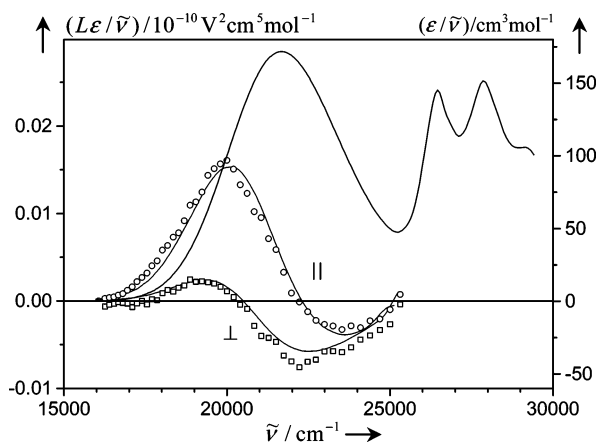
Figure 2. Electrooptical ( L\epsilon/\tilde{\nu} ) and optical ( \epsilon/\tilde{\nu} ) absorption spectra of Hy 9 AN in dioxane solution at T = 298 K. The legend is the same as that in Figure 1.
