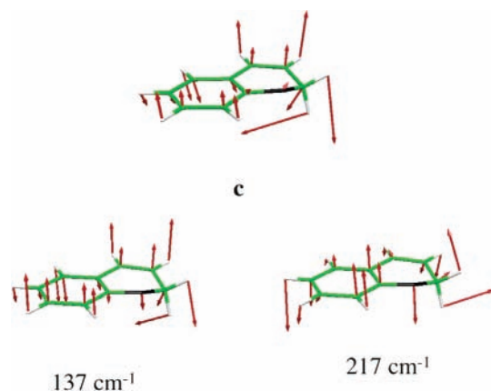
Figure 9. Comparison between patterns of vectors representing the geometry difference between points M and CP (labeled c in Figure 1) and the first (137 cm -1 ) and third (217 cm -1 ) lowest-frequency vibrational modes computed at M for C . The second (145 cm -1 ) lowest-frequency vibration is shown in Figure 6. Note that the 137 and 217 cm -1 vibrations are not FC active.
