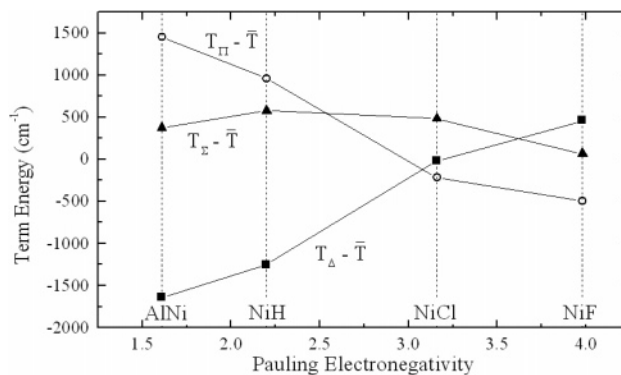
Figure 3. Fitted term energies of the {}^2\Sigma^+ , {}^2\Pi , and {}^2\Delta states of AlNi, NiH, NiCl, and NiF, plotted as a function of the electronegativity of the ligand. A systematic trend is evident.
