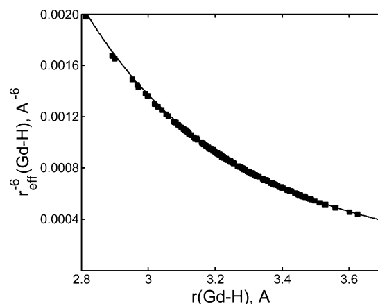
Figure 7. The r_{\text{eff}}^{-6}(\text{Gd-H}) factor for the hydrogen atom of bound water in [\text{Gd}(\text{DOTA})(\text{H}_2\text{O})]^- obtained from eq 10 based on the calculated dipolar HFI tensors of the 100 MD “snapshots” (200 values totally). The line corresponds to r^{-6}(\text{Gd-H}) calculated using the point-dipole approximation.
