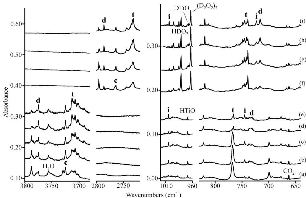
Figure 8. Infrared spectra of the Ti atom and \text{H}_2\text{O}_2 reaction products in excess argon at 10 K. (a) \text{H}_2\text{O}_2 , (b) after annealing to 22 K, (c) after annealing to 26 K, (d) after \lambda > 220 nm irradiation, (e) after annealing to 30 K, (f) \text{D}_2\text{O}_2 , (g) after annealing to 22 K, (h) after \lambda > 220 nm irradiation, and (i) after annealing to 34 K.
