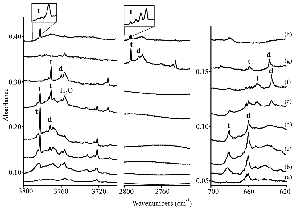
Figure 5. Infrared spectra of the Zr atom and \text{H}_2 + \text{O}_2 reaction products in excess argon at 10 K. (a) \text{H}_2 + {}^{16}\text{O}_2 deposited, (b) after \lambda > 220 nm irradiation, (c) after annealing to 19 K, and (d) after annealing to 24 K and infrared spectra of the following isotopic systems after irradiation and annealing to 22, 23, 28, and 26 K, respectively, (e) \text{H}_2 + {}^{16}\text{O}_2 + {}^{16}\text{O}^{18}\text{O} + {}^{18}\text{O}_2 , (f) \text{H}_2 + {}^{18}\text{O}_2 , (g) \text{D}_2 + {}^{16}\text{O}_2 , and (h) \text{H}_2 + \text{D}_2 + {}^{16}\text{O}_2 .
