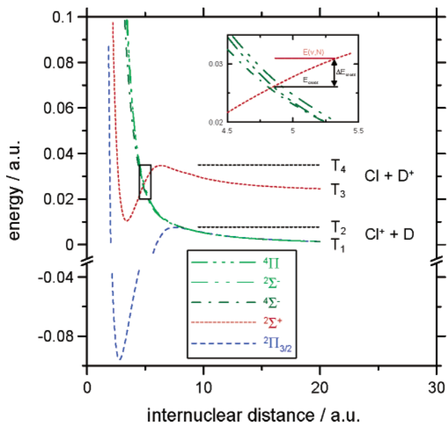
Figure 1. Rotronic potential curves ( N_A = 61 ) of the DCl + ion relevant for the predissociation dynamics, based on data from Dalgarno et al. 32 The inset shows an enlarged view of the crossing region (also marked by a box in the main figure).
