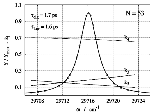
Figure 8. Product ion yield spectrum obtained via the final state \nu_A = 8 , N_A = 53 of \text{DCI}^+ : (symbols) numerical data; (line) Lorentzian function. Relative contribution of the three repulsive states to the overall predissociation process as a function of the excitation frequency (labeled k_3 , k_4 , and k_5 ).
