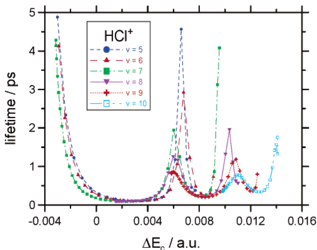
Figure 5. Predissociation lifetime of \text{HCl}^+ in the \nu_A = 5 –10 states as a function of the energy difference between the rovibrational state and the zero-order crossing of the rotronic potentials.
