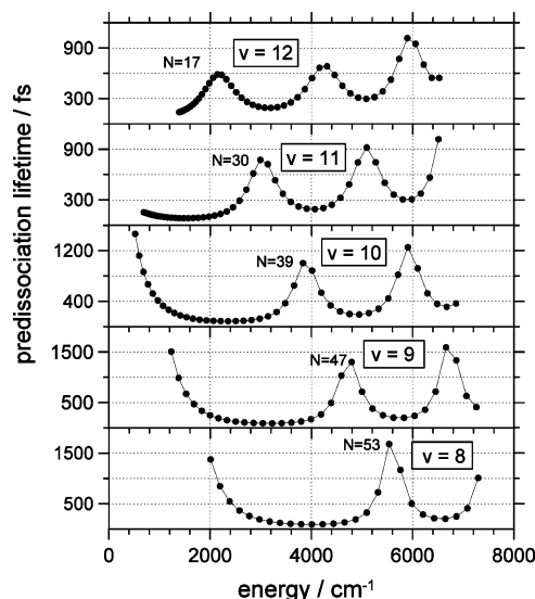
Figure 2. Predissociation lifetime of \text{DCI}^+ in the \nu_A = 8-12 states as a function of the rotational energy relative to the predissociation threshold.
