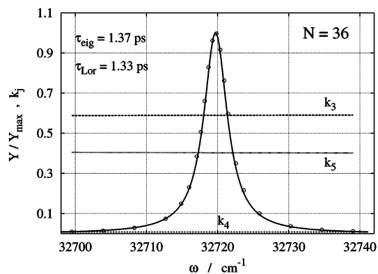
Figure 6. Product yield spectrum obtained via the final state \nu_A = 8 , N_A = 36 of \text{DCI}^+ : (symbols) numerical data; (line) Lorentzian function. Relative contribution of the three repulsive states to the overall predissociation process as a function of the excitation frequency (labeled k_3 , k_4 , and k_5 ).
