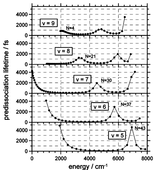
Figure 4. Predissociation lifetime of \text{HCl}^+ in the \nu_A = 5\text{--}9 states as a function of the rotational energy relative to the predissociation threshold.
