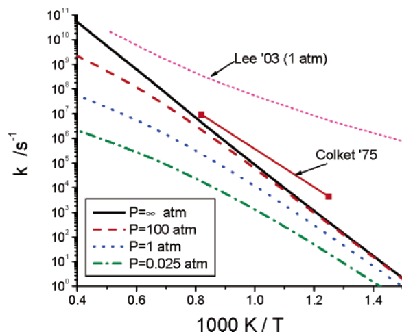
Figure 5. Calculated thermal rate coefficients for the decomposition of vinyoxy radicals as a function of pressure of Ar collider bath. Also shown are results from previous studies. 19,20
