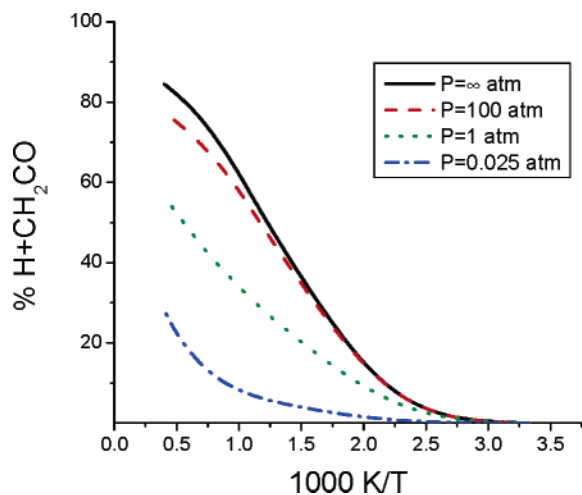
Figure 6. Fraction of the total rate coefficient for dissociation of vinoxy radicals leading to H + ketene at several pressures of Ar collider.
