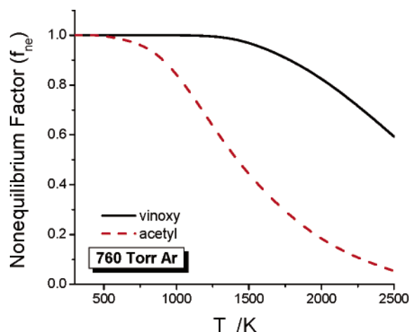
Figure 10. Calculated nonequilibrium ( f_{\text{ne}} ) factor for vinyloxy and acetyl decomposition at 1 atm Ar.
