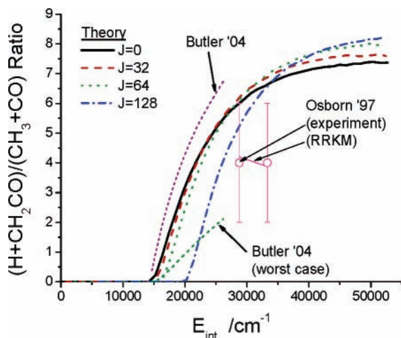
Figure 4. Ratio of rate coefficients leading to H + CH 2 CO and CO + CH 3 , calculated for several values of the angular momentum quantum number (lines). Experimental ratios from the work of Osborn et al. 13 are shown with symbols. Ratios from RRKM calculations of Osborn et al. 13 and Butler et al. 15 are shown with lines.
