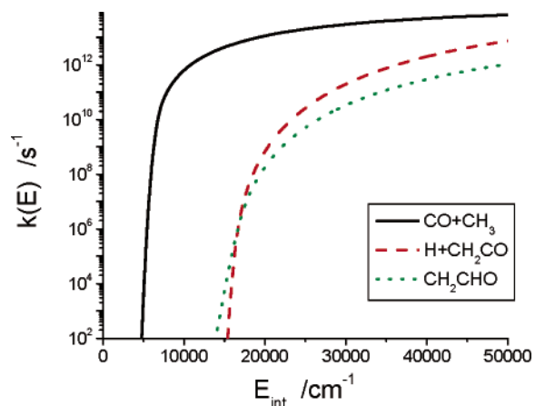
Figure 8. Calculated E-resolved rate coefficients for the decomposition pathways of acetyl radical.
