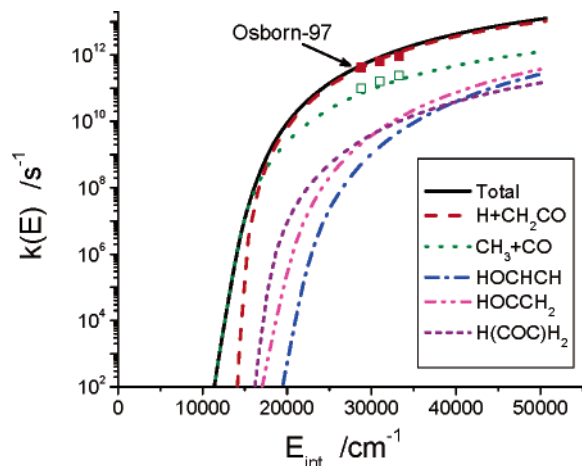
Figure 3. Calculated E-resolved rate coefficients for the decomposition pathways of vinyoxy. Calculations by Osborn et al. 13 for H + CH 2 CO and CO + CH 3 channels are shown with solid and open symbols, respectively.
