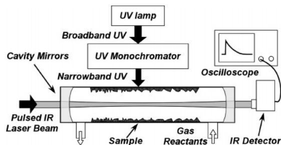
Figure 1. Experimental setup. Quartz flow tube coated with a sample of interest is exposed to gas reactants and/or tunable UV radiation. Gas-phase products are detected using IR CRDS along the flow tube axis.
