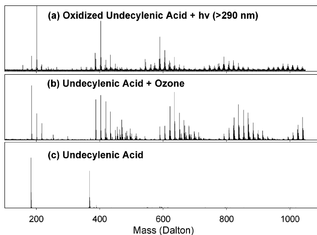
Figure 7. Negative ion electrospray mass-spectra of: (a) undecylenic acid film subjected to ozonolysis and then to photolysis ( \lambda > 295 nm) in dry air; (b) oxidized undecylenic acid; (c) pure undecylenic acid.
