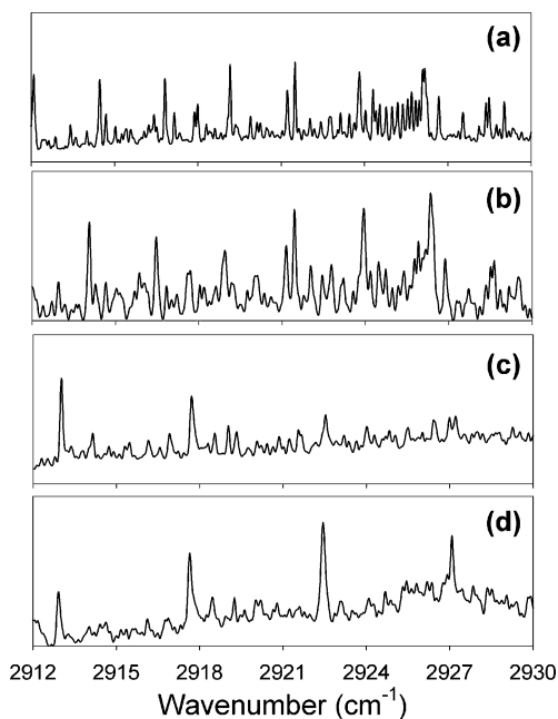
Figure 5. CRDS spectra taken during ozonolysis and subsequent photolysis of undecylenic acid: (a) reference spectrum of formaldehyde convoluted to the CRDS laser line width; (b) CRDS spectrum taken during the ozonolysis; (c) CRDS spectrum taken during UV photolysis of oxidized undecylenic acid; (d) reference optoacoustic spectrum of formic acid taken in parallel with CRDS.
