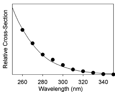
Figure 6. Comparison of action photodissociation (filled circles) and absorption (solid line) spectra of oxidized undecylenic acid. The action spectrum was arbitrarily scaled to fit the absorption data.
