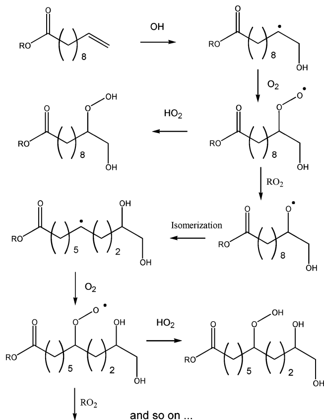
Figure 9. Proposed mechanism for the formation of additional peroxy bonds in the oxidized sample. OH and HO 2 come from decomposition of carbonyl oxide (III).
