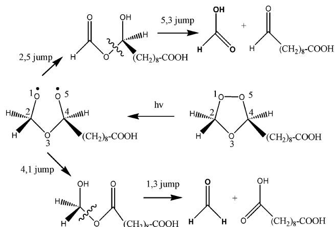
Figure 10. One of the possible mechanisms of photolytic production of HCHO and HCOOH from the oxidized undecylenic acid. Preferential formation of HCOOH can be explained by steric hindrance in the H-transfer step.
