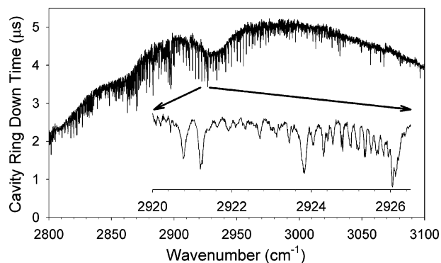
Figure 4. CRDS spectrum of the gas-phase oxidation products of undecylenic acid. The fine structure is due to formaldehyde, and the overall shape of the spectrum is due to the reflectivity profile of the cavity mirrors. Present experiments use the narrow window between 2920 and 2927 \text{cm}^{-1} showed in the enlarged region.
