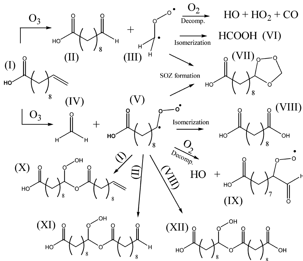
Figure 8. Primary reactions taking place during ozonolysis of undecylenic acid film. Products (II, IV, VI, VIII, X, XI, XII) could be observed directly. SOZ (VII) and carbonyl oxides (III, V) participate in secondary reactions such as decomposition and oligomerization (not shown).
