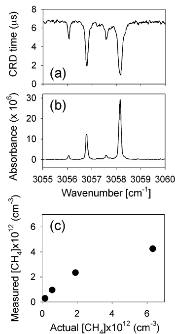
Figure 2. Characterization of the CRDS setup. (a) Cavity ring-down time measured with 1.4 \times 10^{13} molecule/ \text{cm}^3 of \text{CH}_4 in the cell. (b) Absorbance calculated from the ring-down time. (c) Measured and actual density of \text{CH}_4 . The observed nonlinearity is due to the low spectral resolution of the pump laser.
