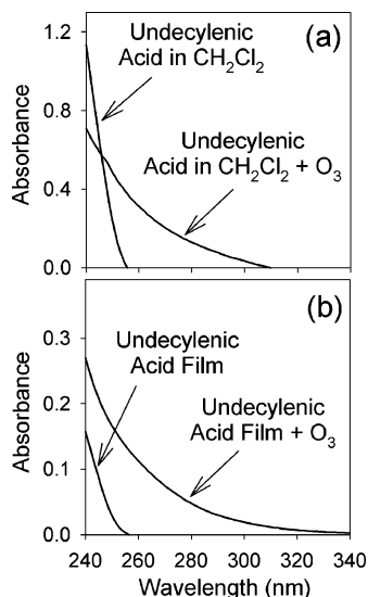
Figure 3. UV absorption spectra of undecylenic acid and its oxidation products. The ozonolysis reaction was carried out: (a) in the liquid phase; (b) on the surface of a thin multilayered film.
