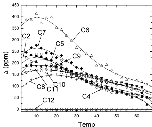
Figure 9. 13 C CSA ( \Delta ) for [EMIM]BSO 3 ionic liquid vs temperature. Imidazolium ring 13 C's: C2, 139.9 ppm (●); C4, 124.0 ppm (○); C5, 122.5 ppm (▲). Ring methyl 13 C: C6, 35.9 ppm (△). Ring methylene 13 C: C7, 44.6 ppm (◆). Terminal methyl 13 C: C8, 15.6 ppm (+). Butanesulfonate 13 C's: SO 3 methylene 13 C, C9, 51.9 ppm (▼); methylene 13 C, C10, 27.9 ppm (▽); methylene 13 C, C11, 22.1 ppm (⊙); terminal methyl 13 C, C12, 13.9 ppm (×).
