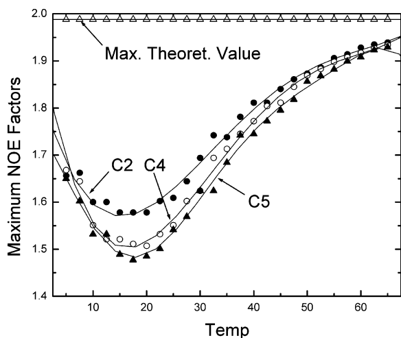
Figure 4. Corrected maximum 13 C NOE factors and total spin–lattice relaxation times ( T 1 's). For [MNIM]PF 6 ionic liquid vs temperature: (●) imidazolium ring C2 carbon; (○) imidazolium ring C4 and (▲) C5 carbons; (Δ) theoretical NOE 13 C maximum of 1.988.
