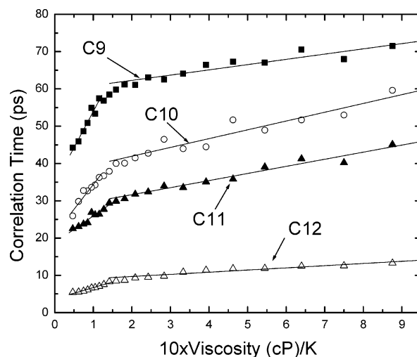
Figure 8. Correlation time (ps) for butyl carbons in BSO 3 in [EMIM]-SO 3 vs viscosity/K (cP/K): C9 (■); C10 (○); C11 (▲); C12 (△). From left to right, temperature ranges include approximately 328–303 K and 303–278 K.
