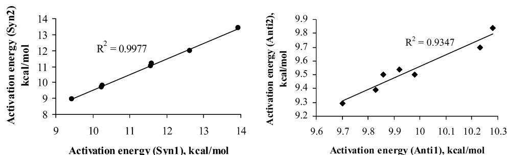
Figure 6. Correlation between Syn1 and Syn2 barriers as well as Anti1 and Anti2 barriers calculated from the hydrogen abstractions of ortho-substituted 1,4-didehydronaphthalene at the UB3LYP/6-31G** level.
