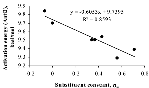
Figure 9. Correlation between Hammett constants ( \sigma_m ) and the activation barriers for the anti type hydrogen abstractions at the UB3LYP/6-31G** level.
