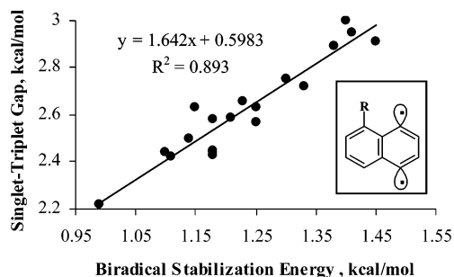
Figure 3. Correlation of two estimates of substituent effects on electronic coupling of radical centers in p -naphthyl diradicals at the UB3LYP/6-31G** level.
