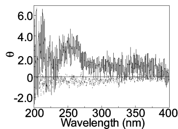
Figure 3. ICD signal of Fis in the presence of 12 mM \beta -CD (—) and in water (···).
