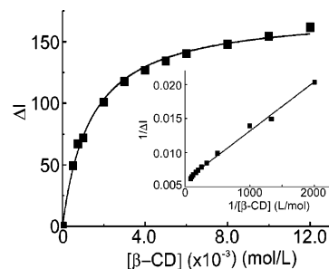
Figure 2. Representative plot of the variation in fluorescence intensity as a function of \beta -CD concentration as analyzed by the Benesi–Hildebrand equation 9 at 530 nm. Inset: the double-reciprocal plot.
